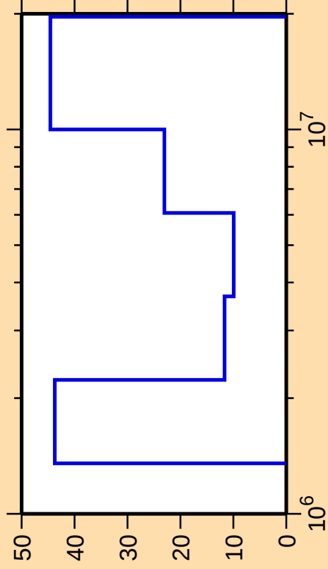
\Delta\sigma/\sigma vs. E for ^{183}\text{Ta}(n,\text{ncont.})
