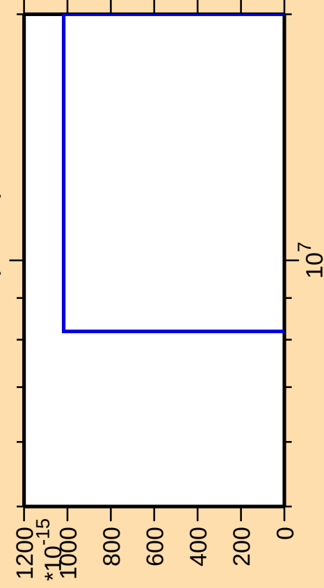
\Delta\sigma/\sigma vs. E for ^{183}\text{Ta}(\text{mt } 42)
