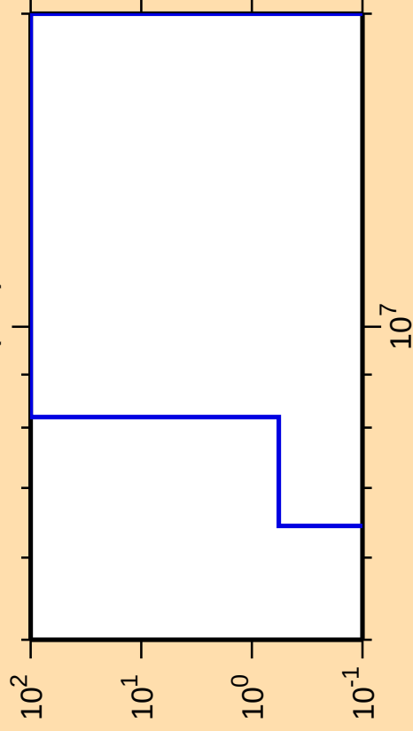
\Delta\sigma/\sigma vs. E for ^{183}\text{Ta}(n,d)
