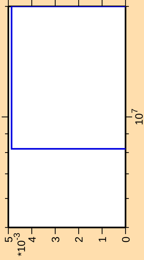
\Delta\sigma/\sigma vs. E for ^{183}\text{Ta}(n,3n\alpha)
