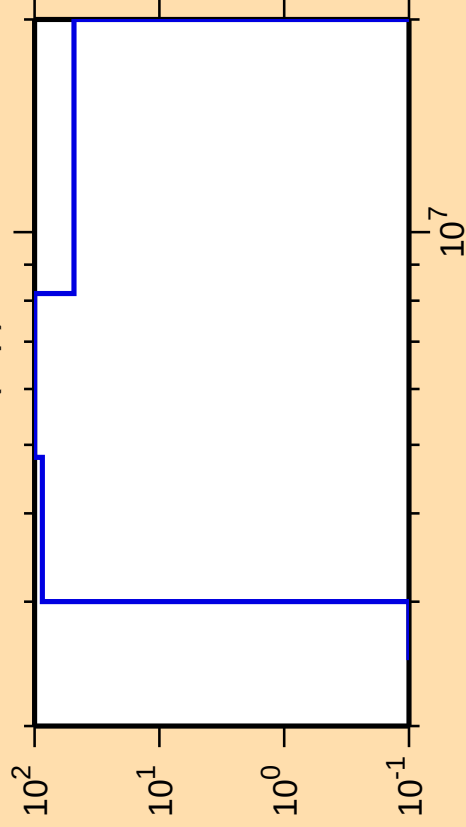
\Delta\sigma/\sigma vs. E for ^{183}\text{Ta}(n,p)
