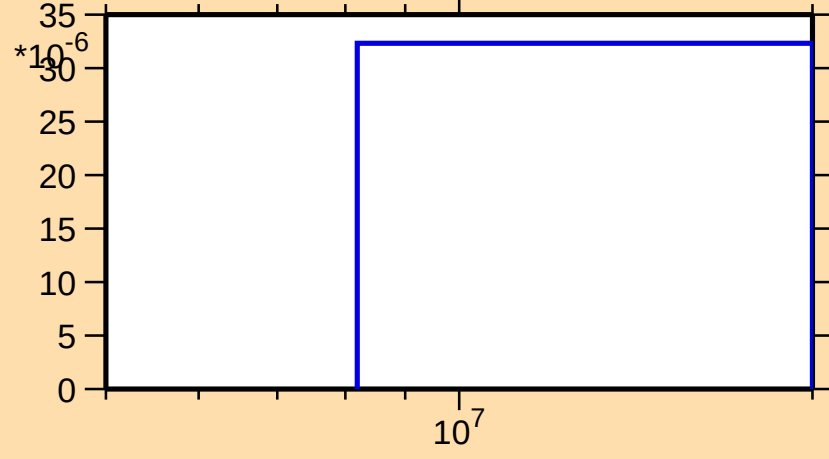
\sigma vs. E for ^{183}\text{Ta}(n,t)
