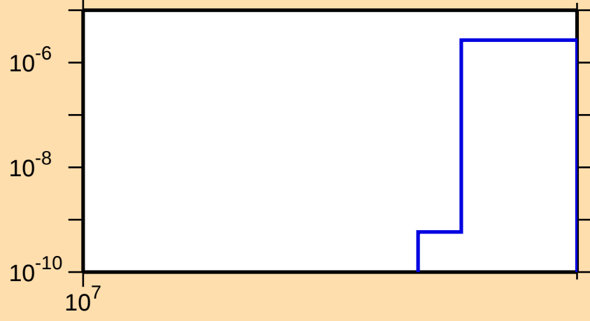
\sigma vs. E for ^{87}\text{Tc}(n,2np)
