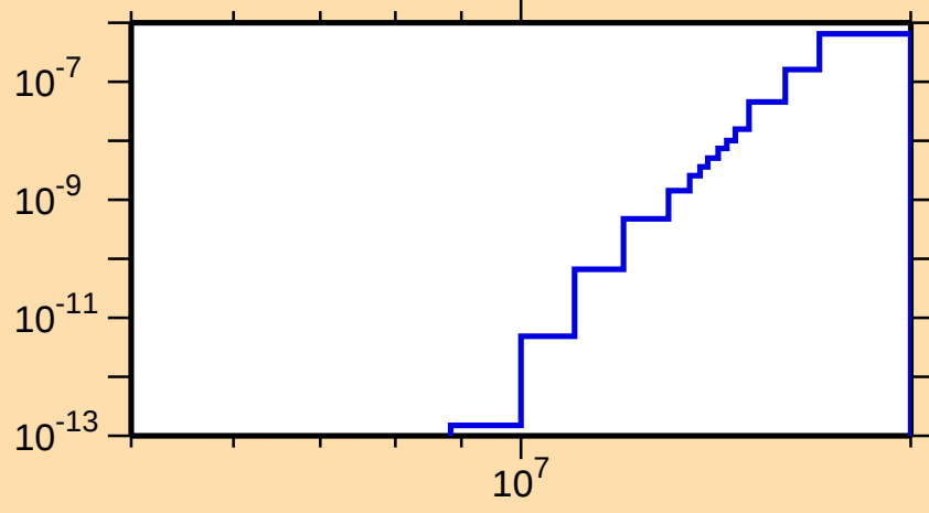
\sigma vs. E for ^{87}\text{Tc}(\text{mt117})
