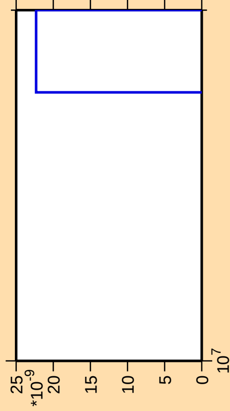
\Delta\sigma/\sigma vs. E for ^{87}\text{Tc}(n,\text{nt})
