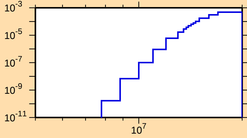
\sigma vs. E for ^{87}\text{Tc}(n,\alpha)
