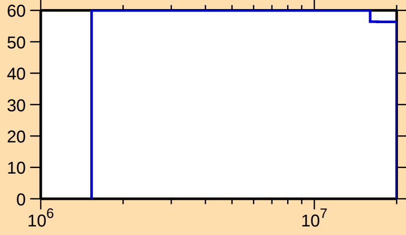
\Delta\sigma/\sigma vs. E for ^{87}\text{Tc}(n,n\text{cont.})
