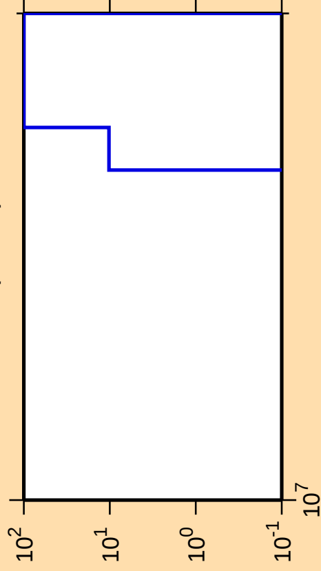
\Delta\sigma/\sigma vs. E for ^{87}\text{Tc}(\text{mt } 34)
