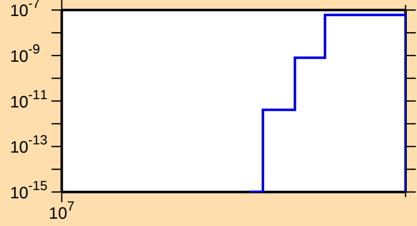
\sigma vs. E for ^{87}\text{Tc}(n,\text{nd})
