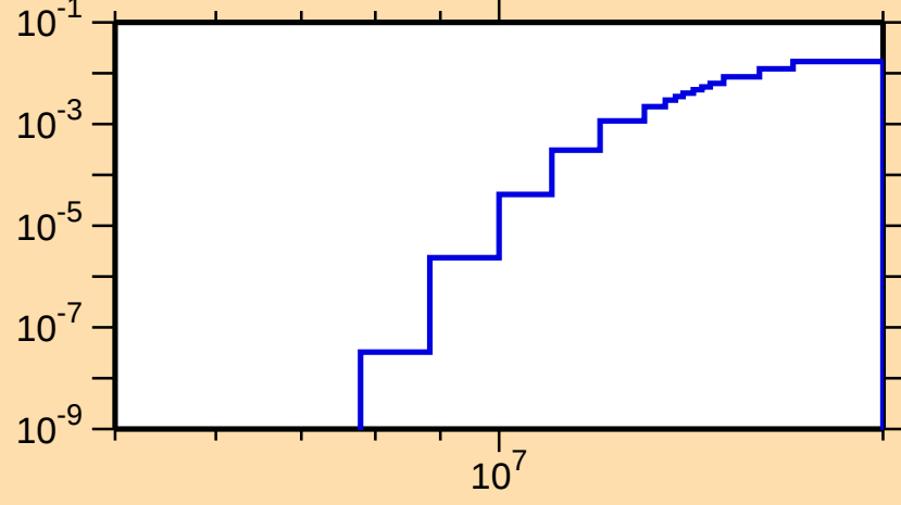
\sigma vs. E for ^{87}\text{Tc}(n,\text{pd})
