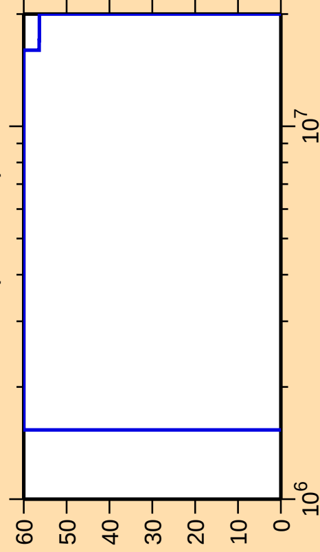
\Delta\sigma/\sigma vs. E for ^{87}\text{Tc}(n,\text{ncont.})
