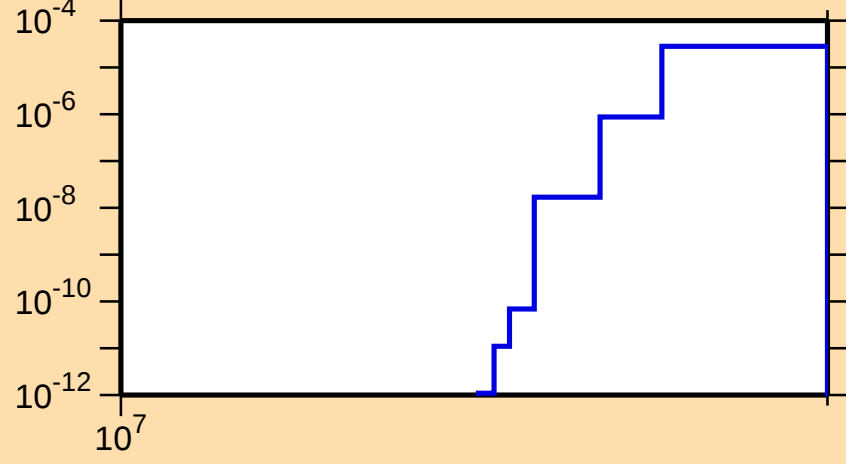
\sigma vs. E for ^{87}\text{Tc}(n,\text{pt})
