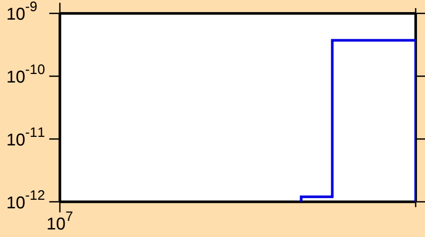
\sigma vs. E for ^{87}\text{Tc}(\text{mt } 34)
