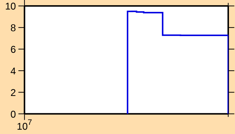
\Delta\sigma/\sigma vs. E for ^{87}\text{Tc}(n,\text{inel.})
