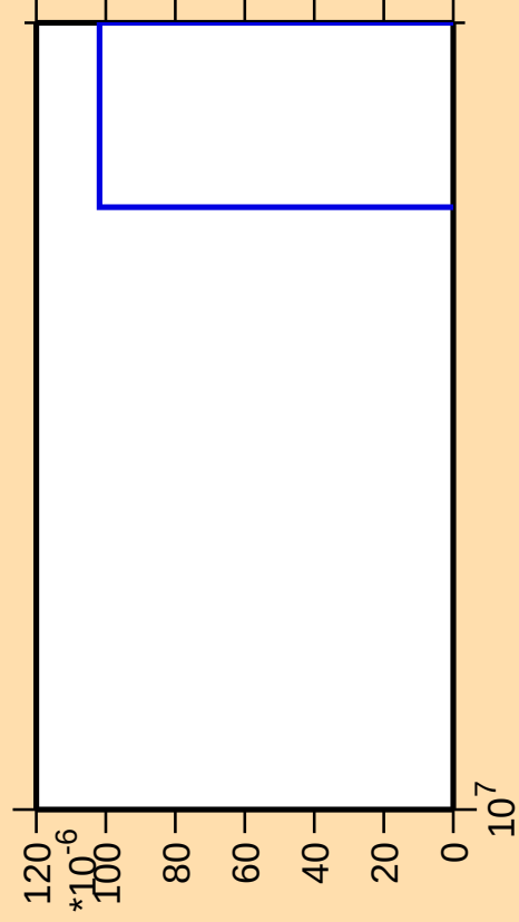
\Delta\sigma/\sigma vs. E for ^{91}\text{Tc}(n,\text{nt})
