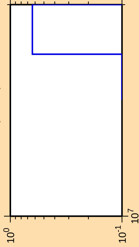
\Delta\sigma/\sigma vs. E for ^{91}\text{Tc}(\text{mt } 34)
