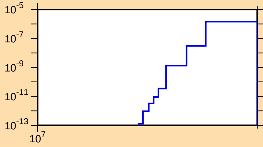
\sigma vs. E for ^{91}\text{Tc}(\text{mt } 45)
