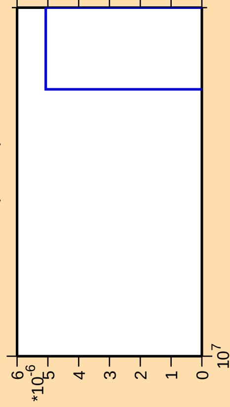
\Delta\sigma/\sigma vs. E for ^{98}\text{Tc}(n,3n\alpha)
