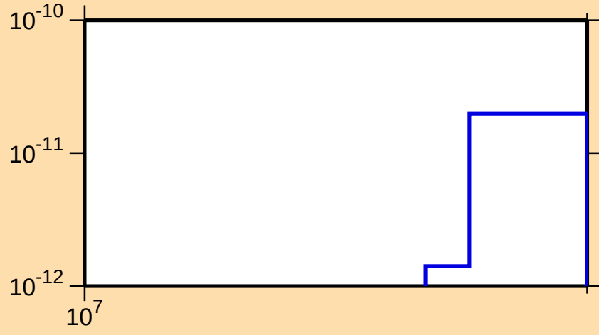
\sigma vs. E for ^{98}\text{Tc}(\text{mt117})
