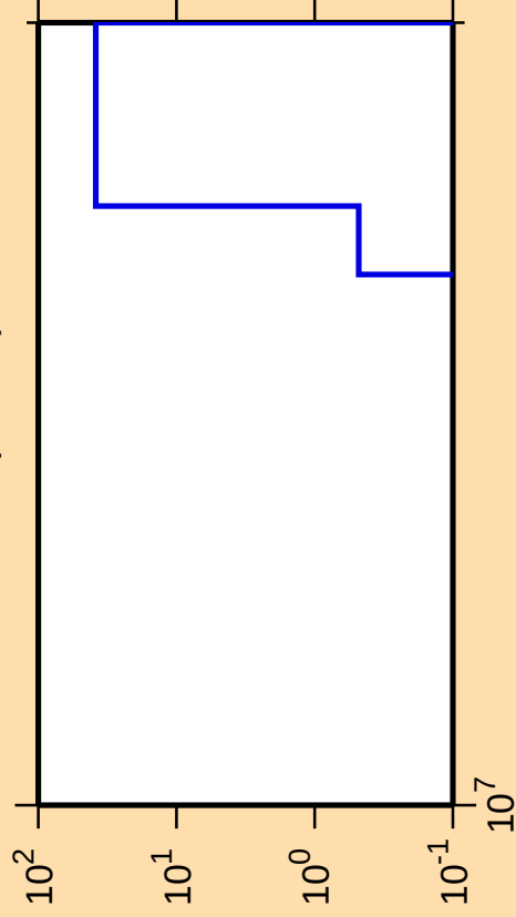
\Delta\sigma/\sigma vs. E for ^{98}\text{Tc}(\text{mt } 45)
