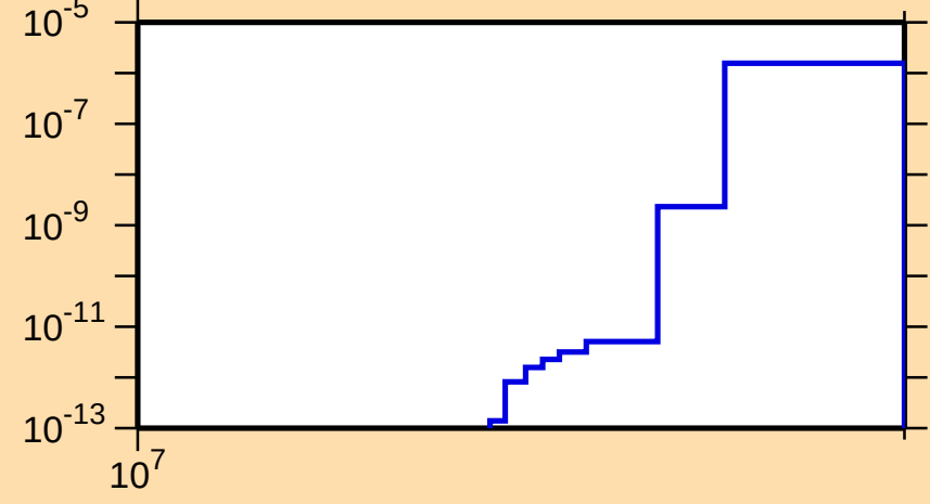
\sigma vs. E for ^{98}\text{Tc}(n,\text{nt})
