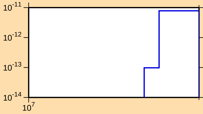
\sigma vs. E for ^{98}\text{Tc}(\text{mt } 45)
