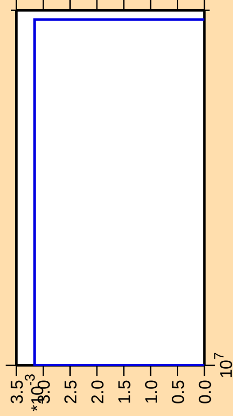
\Delta\sigma/\sigma vs. E for ^{98}\text{Tc}(\text{mt } 34)
