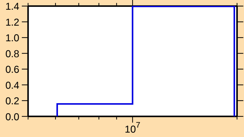
\sigma vs. E for ^{98}\text{Tc}(n,2n)
