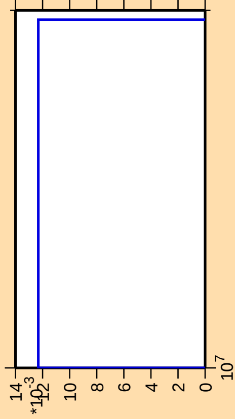
\Delta\sigma/\sigma vs. E for ^{98}\text{Tc}(n,\text{pd})
