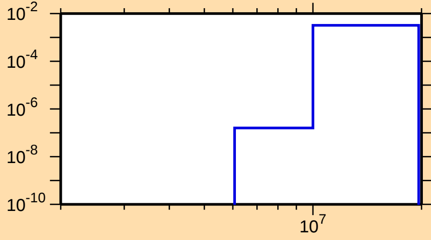
\sigma vs. E for ^{98}\text{Tc}(n,\alpha)
