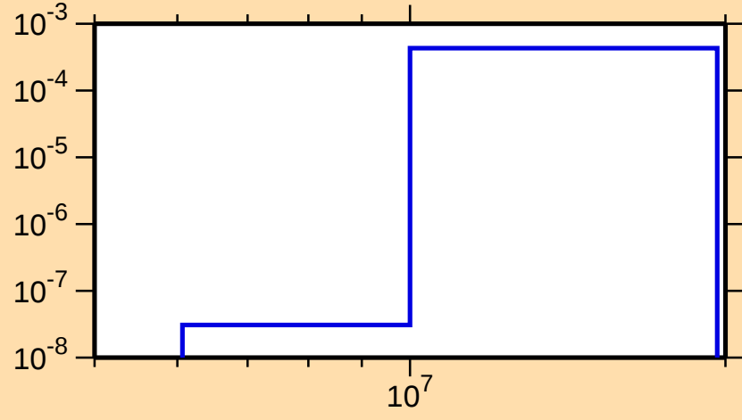
\sigma vs. E for ^{98}\text{Tc}(n,t)
