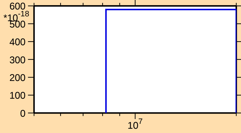
\sigma vs. E for ^{98}\text{Tc}(\text{mt } 34)
