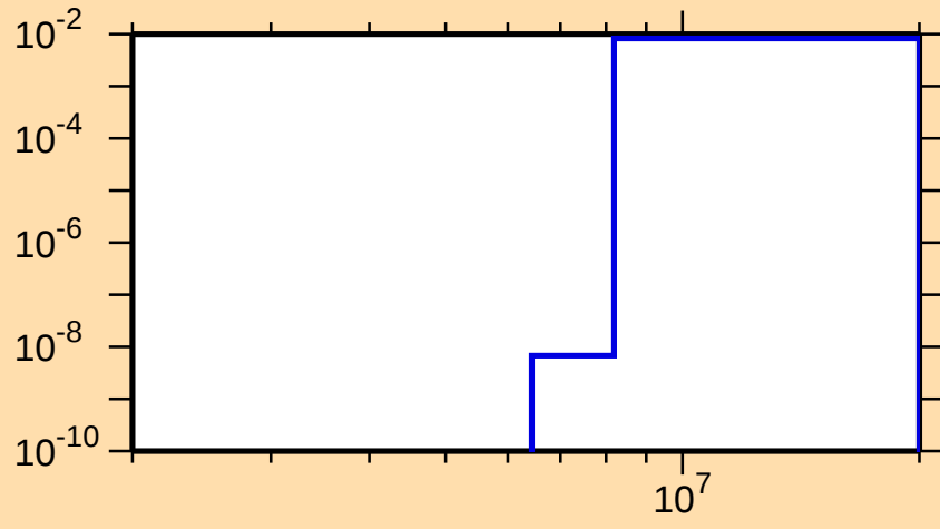
\sigma vs. E for ^{98}\text{Tc}(n,np)
