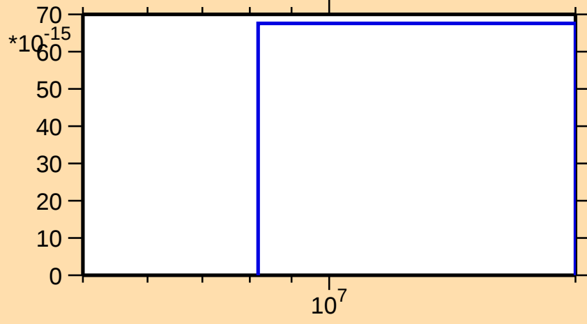
\sigma vs. E for ^{98}\text{Tc}(\text{mt } 45)
