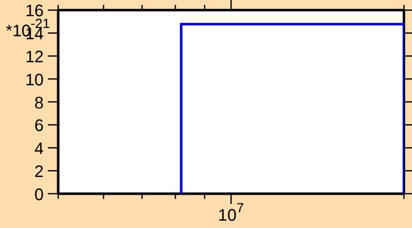
\sigma vs. E for ^{98}\text{Tc}(n,3n\alpha)
