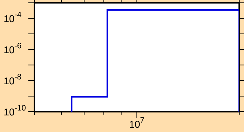
\sigma vs. E for ^{98}\text{Tc}(n,t)
