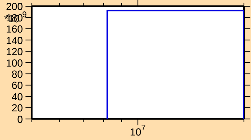
\sigma vs. E for ^{98}\text{Tc}(n,2n\alpha)
