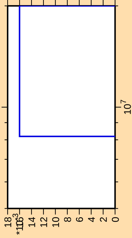
\Delta\sigma/\sigma vs. E for ^{98}\text{Tc}(n,\text{pd})
