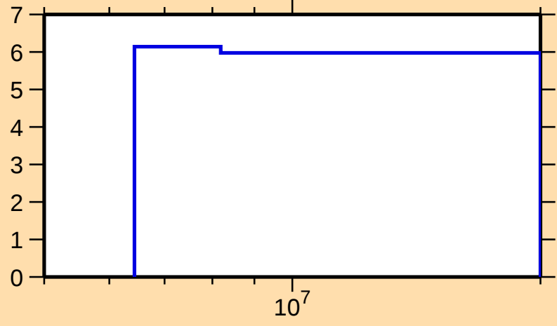
\Delta\sigma/\sigma vs. E for ^{98}\text{Tc}(n,\text{nonel.})
