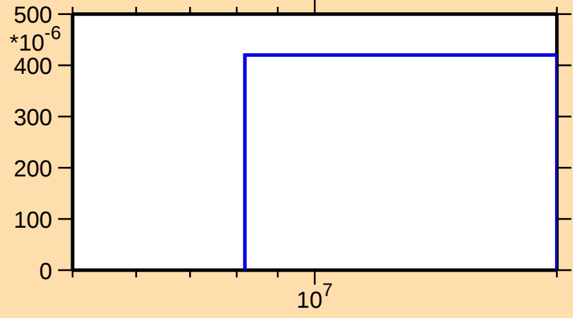
\sigma vs. E for ^{98}\text{Tc}(n,3n)
