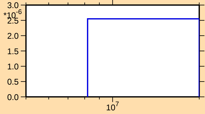
\sigma vs. E for ^{98}\text{Tc}(n,\text{nd})
