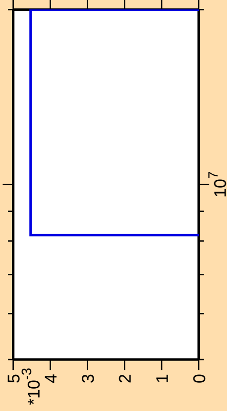
\Delta\sigma/\sigma vs. E for ^{98}\text{Tc}(\text{mt } 34)
