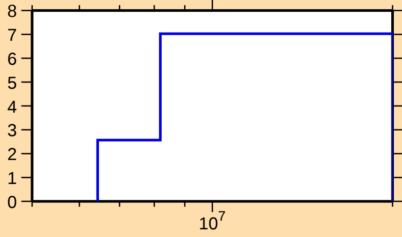
\Delta\sigma/\sigma vs. E for ^{98}\text{Tc}(n,\text{tot.})
