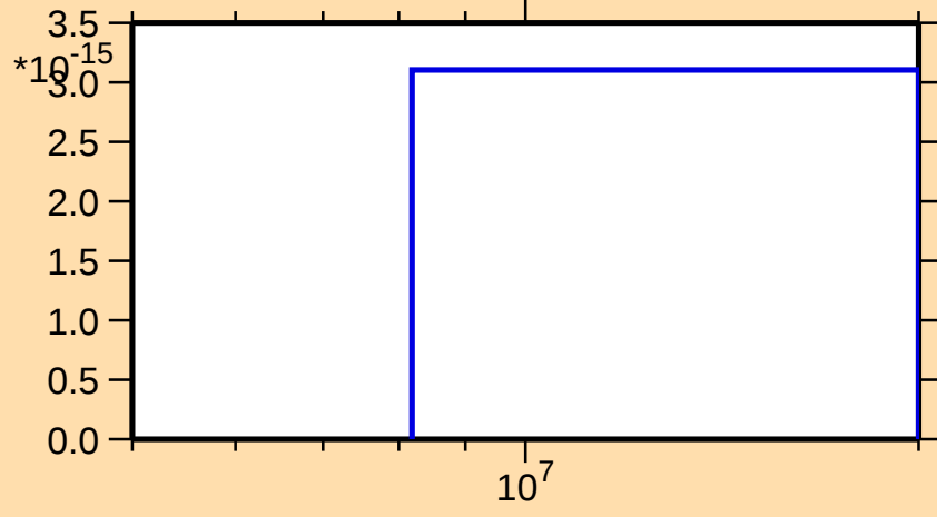
\sigma vs. E for ^{98}\text{Tc}(n,\text{pd})
