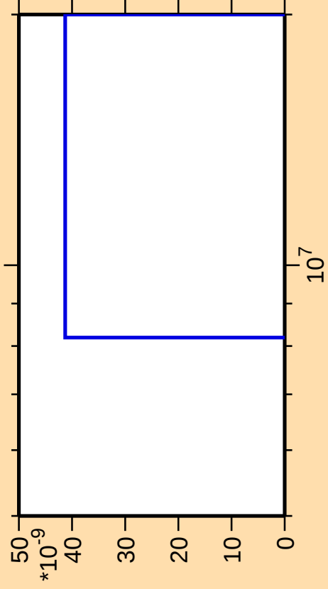
\Delta\sigma/\sigma vs. E for ^{98}\text{Tc}(n,3n\alpha)
