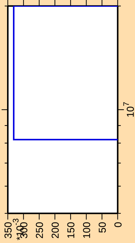
\Delta\sigma/\sigma vs. E for ^{98}\text{Tc}(\text{mt } 45)
