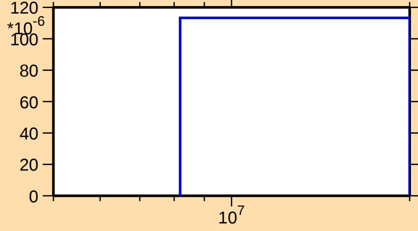
\sigma vs. E for ^{99}\text{Tc}(n,t)
