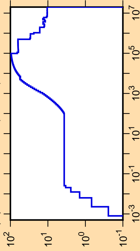
\Delta\mu/\mu vs. E for ^{103}\text{Tc}(\text{mt251})
