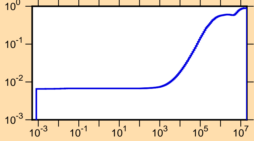
\mu vs. E for ^{103}\text{Tc}(\text{mt251})
