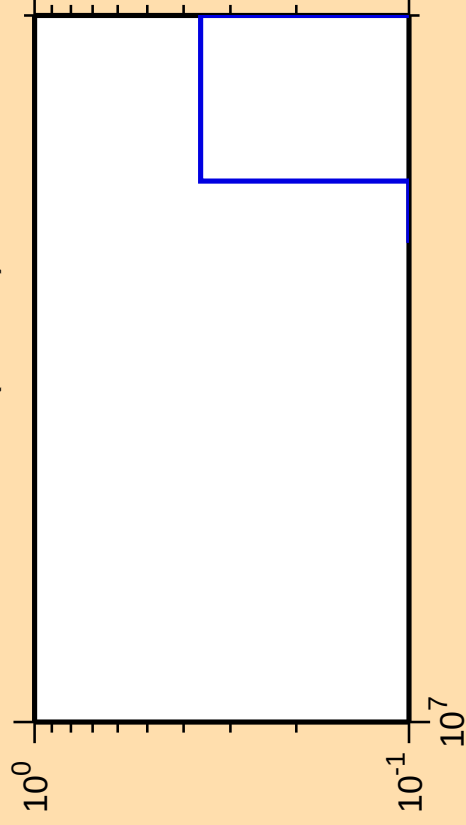
\Delta\sigma/\sigma vs. E for ^{103}\text{Tc}(n,\text{He3})
