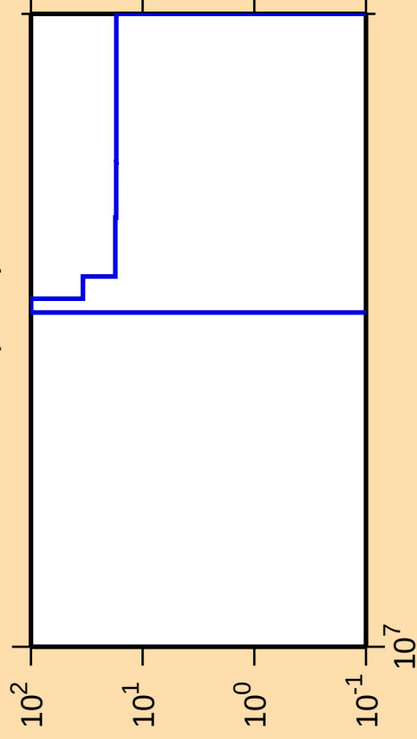
\Delta\sigma/\sigma vs. E for ^{103}\text{Tc}(n,3n)
