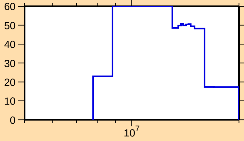
\Delta\sigma/\sigma vs. E for ^{103}\text{Tc}(n,\text{inel.})
