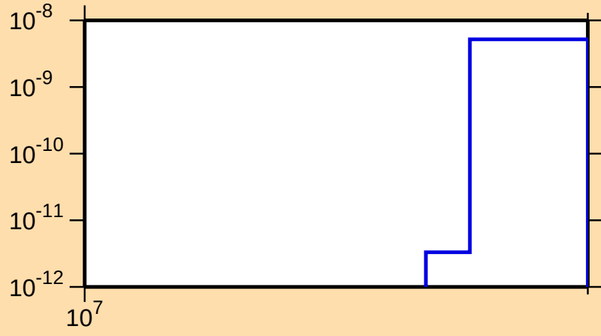
\sigma vs. E for ^{103}\text{Tc}(n,2n\alpha)
