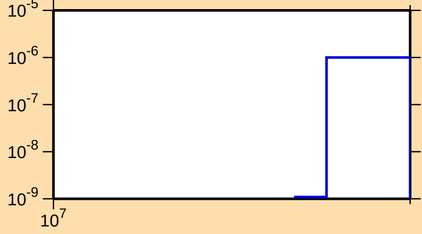
\sigma vs. E for ^{103}\text{Tc}(n,\text{nd})
