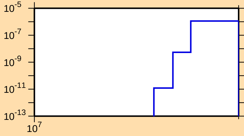
\sigma vs. E for ^{103}\text{Tc}(n,\text{nt})
