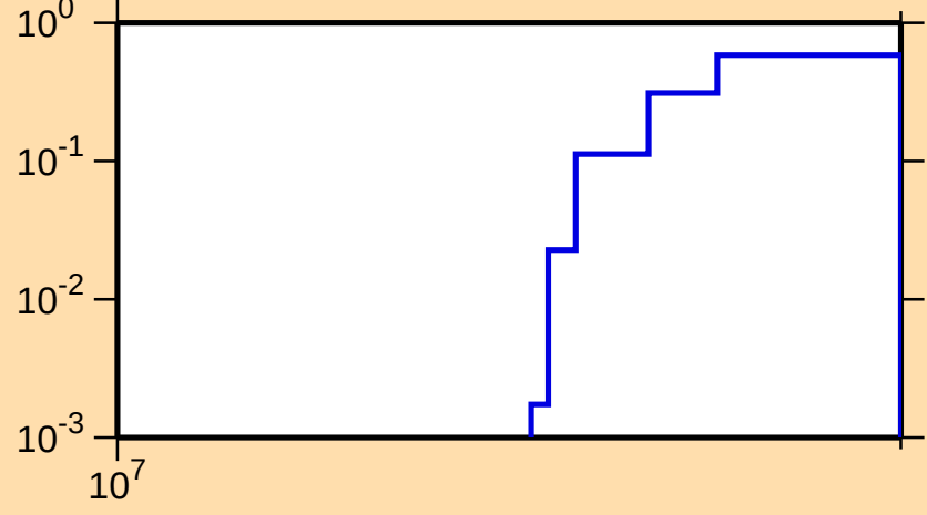
\sigma vs. E for ^{103}\text{Tc}(n,3n)
