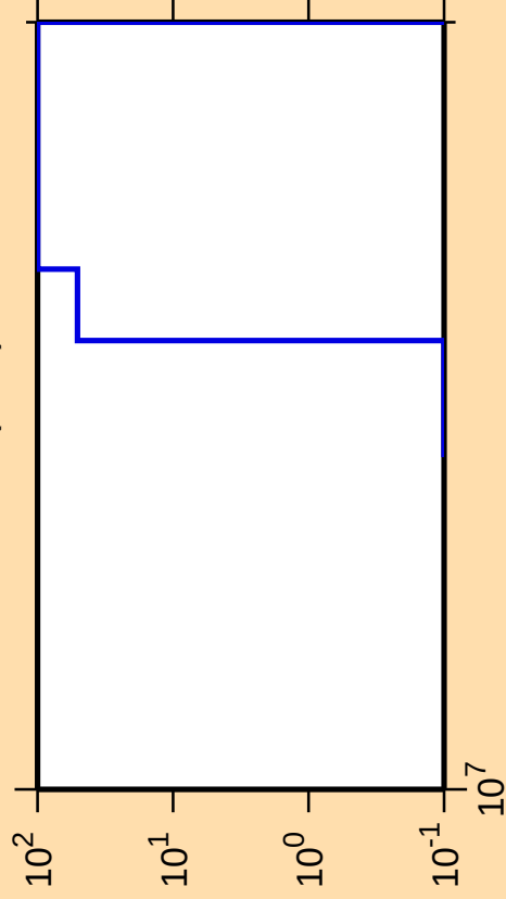
\Delta\sigma/\sigma vs. E for ^{103}\text{Tc}(n,\text{nt})
