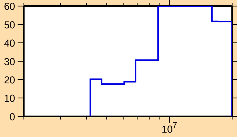
\Delta\sigma/\sigma vs. E for ^{103}\text{Tc}(n,n\text{cont.})
