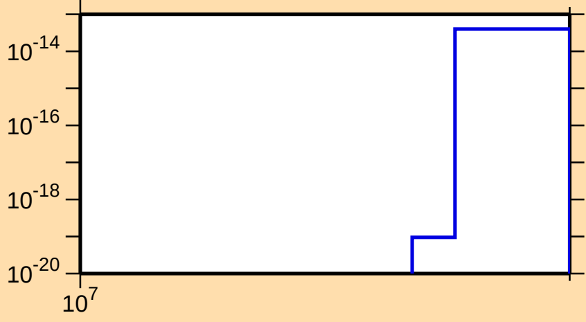
\sigma vs. E for ^{103}\text{Tc}(n,\text{He3})
