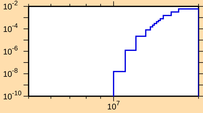
\sigma vs. E for ^{103}\text{Tc}(n,np)
