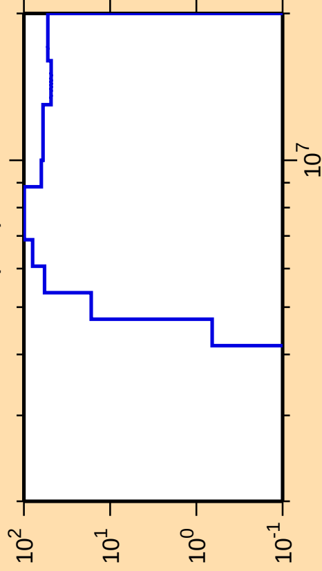
\Delta\sigma/\sigma vs. E for ^{103}\text{Tc}(n,\alpha)
