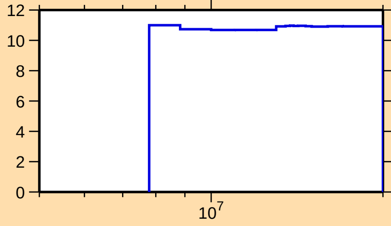
\Delta\sigma/\sigma vs. E for ^{103}\text{Tc}(n,\text{nonel.})
