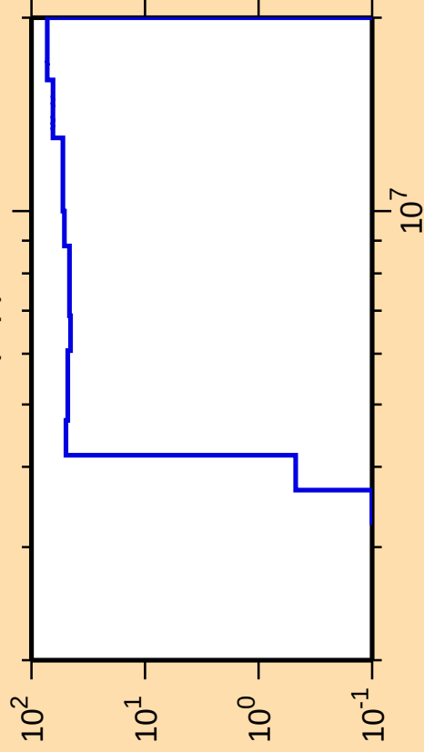
\Delta\sigma/\sigma vs. E for ^{103}\text{Tc}(n,p)
