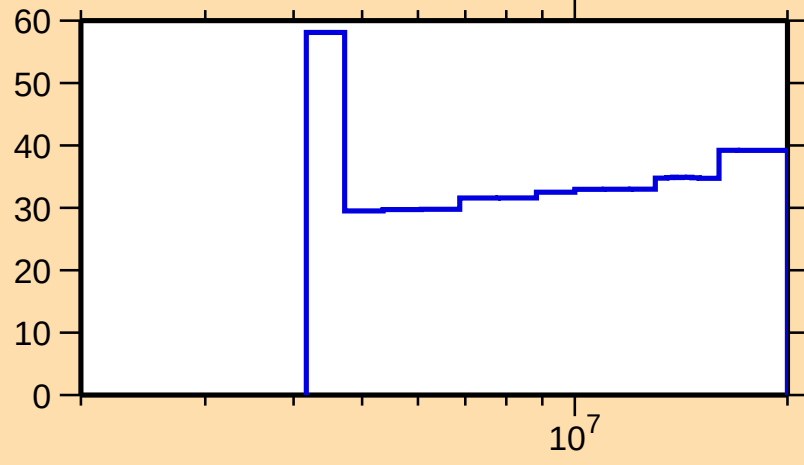
\Delta\sigma/\sigma vs. E for ^{103}\text{Tc}(n,n_1)
