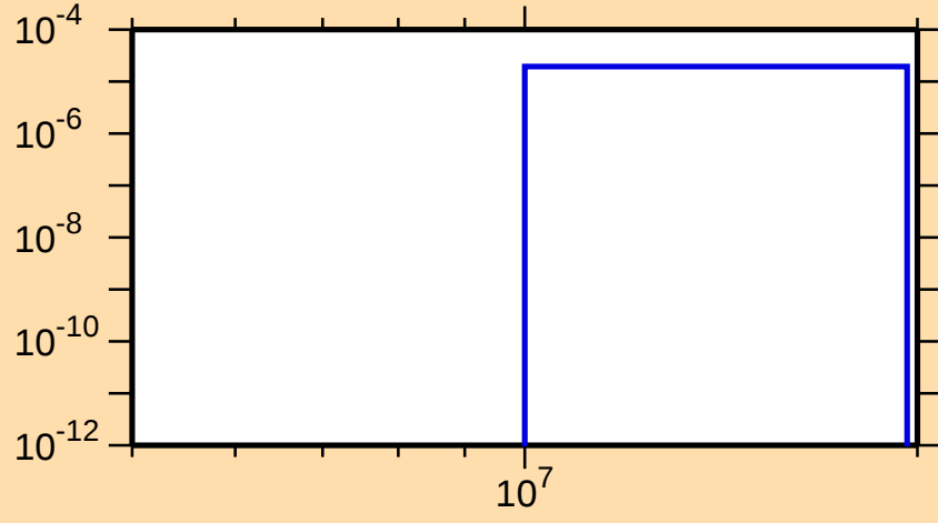
\sigma vs. E for ^{103}\text{Tc}(n,t)
