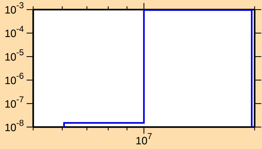
\sigma vs. E for ^{103}\text{Tc}(n,d)
