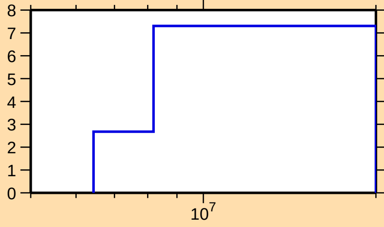
\Delta\sigma/\sigma vs. E for ^{103}\text{Tc}(n,\text{tot.})
