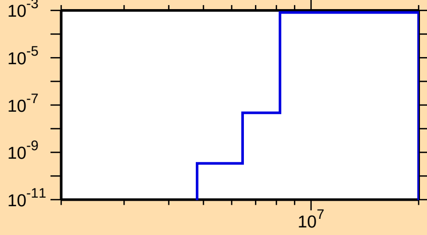
\sigma vs. E for ^{103}\text{Tc}(n,\alpha)
