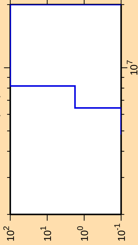
\Delta\sigma/\sigma vs. E for ^{103}\text{Tc}(n,d)
