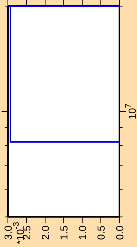
\Delta\sigma/\sigma vs. E for ^{103}\text{Tc}(n,\text{He3})
