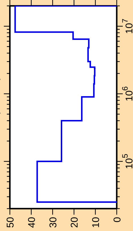
\Delta\sigma/\sigma vs. E for ^{103}\text{Tc}(n,\text{inel.})
