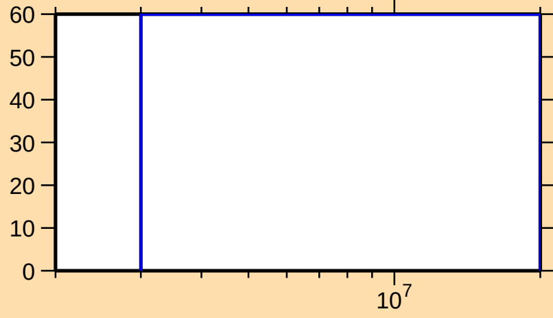
\Delta\sigma/\sigma vs. E for ^{103}\text{Tc}(n,\gamma)
