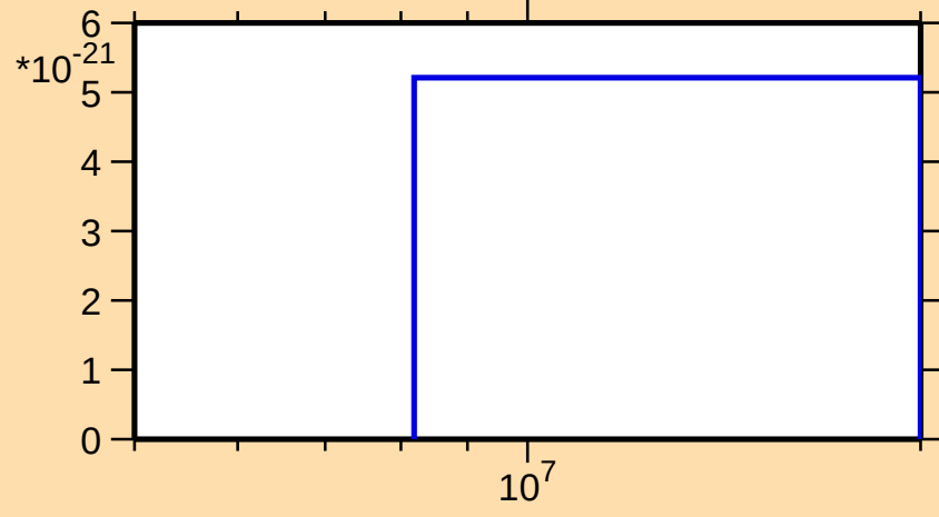
\sigma vs. E for ^{103}\text{Tc}(\text{mt } 11)
