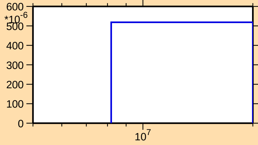
\sigma vs. E for ^{103}\text{Tc}(n,np)
