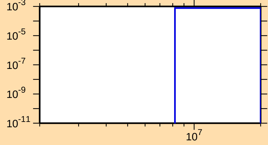
\sigma vs. E for ^{103}\text{Tc}(n,d)
