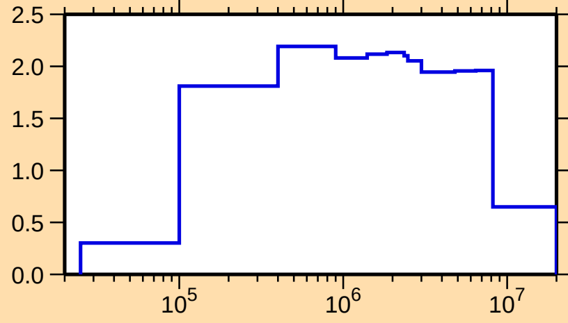
\sigma vs. E for ^{103}\text{Tc}(n,\text{inel.})
