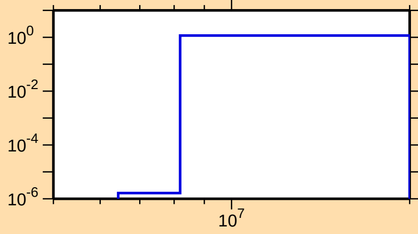
\sigma vs. E for ^{103}\text{Tc}(n,2n)
