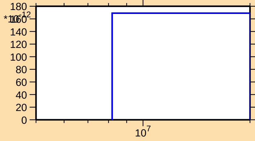
\sigma vs. E for ^{103}\text{Tc}(n,2np)
