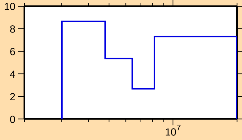
\Delta\sigma/\sigma vs. E for ^{103}\text{Tc}(n,\text{tot.})
