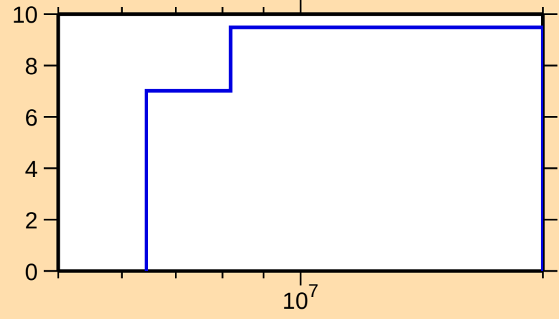
\Delta\sigma/\sigma vs. E for ^{103}\text{Tc}(n,\text{el.})
