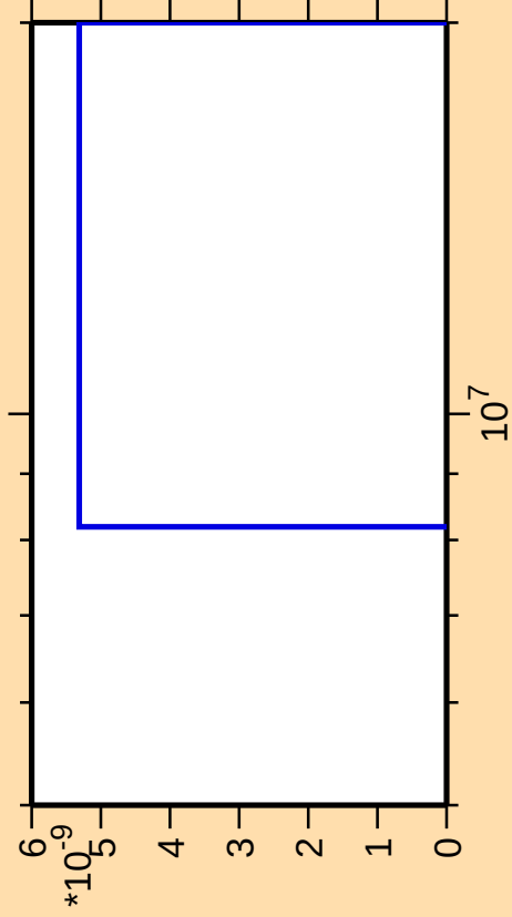
\Delta\sigma/\sigma vs. E for ^{103}\text{Tc}(\text{mt } 11)
