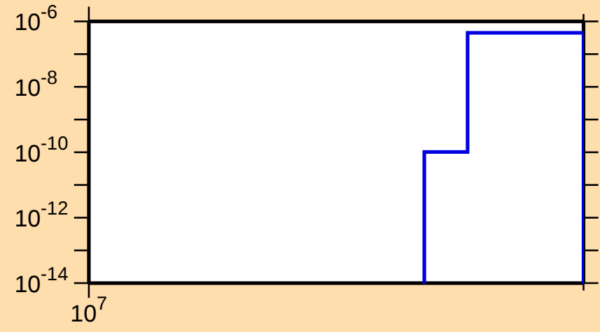
\sigma vs. E for ^{107}\text{Tc}(n,\text{nd})
