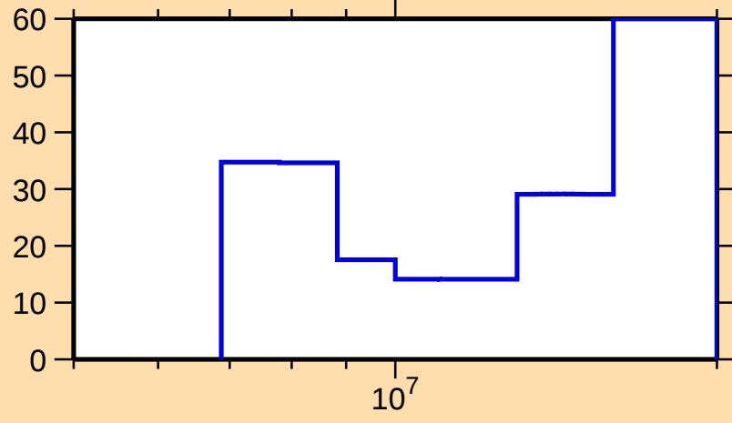
\Delta\sigma/\sigma vs. E for ^{107}\text{Tc}(n,2n)
