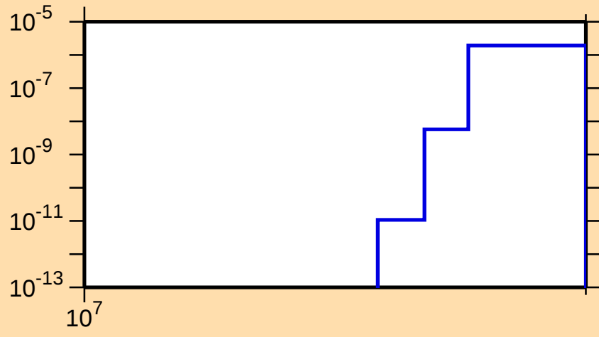
\sigma vs. E for ^{107}\text{Tc}(n,nt)
