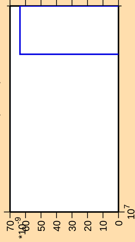
\Delta\sigma/\sigma vs. E for ^{107}\text{Tc}(\text{mt } 11)
