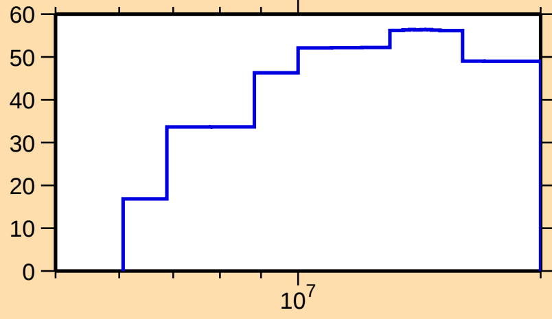
\Delta\sigma/\sigma vs. E for ^{107}\text{Tc}(n,\text{inel.})
