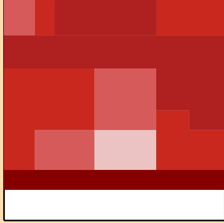
\Delta\sigma/\sigma vs. E for ^{107}\text{Tc}(n,n_1)
