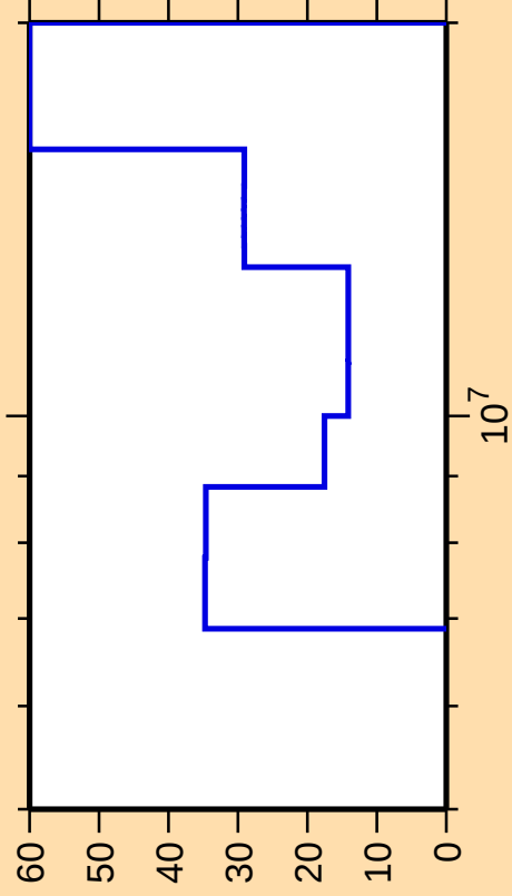
\Delta\sigma/\sigma vs. E for ^{107}\text{Tc}(n,2n)
