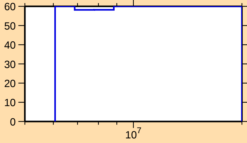
\Delta\sigma/\sigma vs. E for ^{107}\text{Tc}(n,\gamma)
