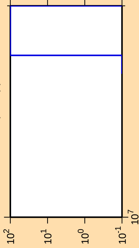
\Delta\sigma/\sigma vs. E for ^{107}\text{Tc}(n,2np)
