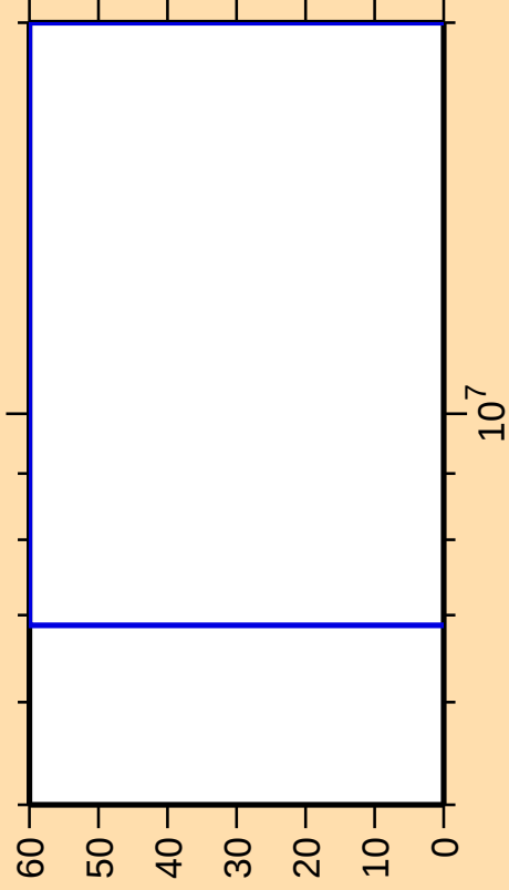
\Delta\sigma/\sigma vs. E for ^{107}\text{Tc}(n,n_1)
