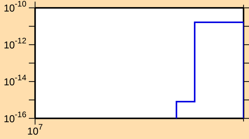
\sigma vs. E for ^{107}\text{Tc}(n,2n\alpha)
