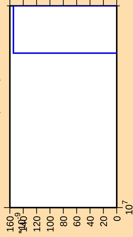
\Delta\sigma/\sigma vs. E for ^{107}\text{Tc}(n,3n\alpha)
