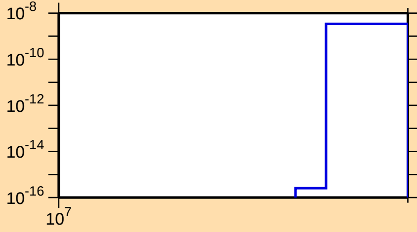
\sigma vs. E for ^{107}\text{Tc}(n,2np)
