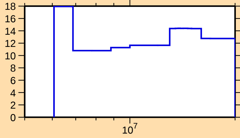
\Delta\sigma/\sigma vs. E for ^{107}\text{Tc}(n,\text{nonel.})
