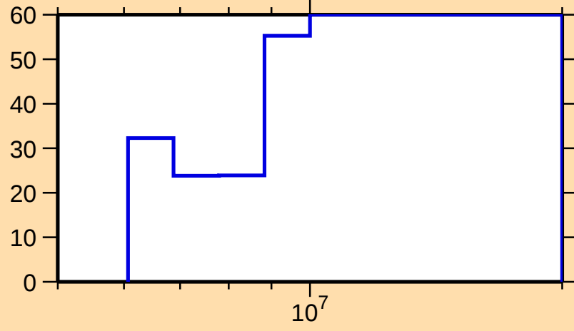
\Delta\sigma/\sigma vs. E for ^{107}\text{Tc}(n,n\text{cont.})
