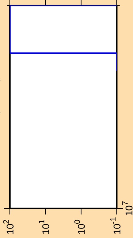
\Delta\sigma/\sigma vs. E for ^{107}\text{Tc}(n,2n\alpha)
