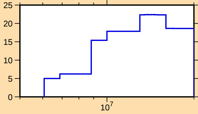
\Delta\sigma/\sigma vs. E for ^{107}\text{Tc}(n,\text{tot.})
