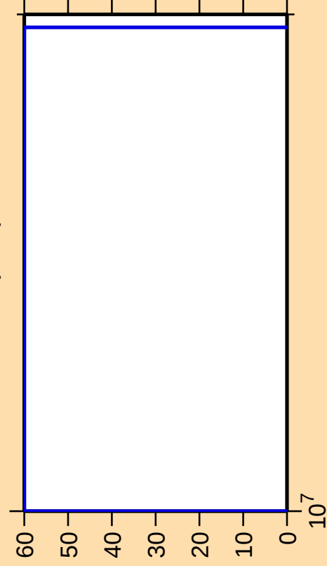
\Delta\sigma/\sigma vs. E for ^{107}\text{Tc}(n,\text{nt})
