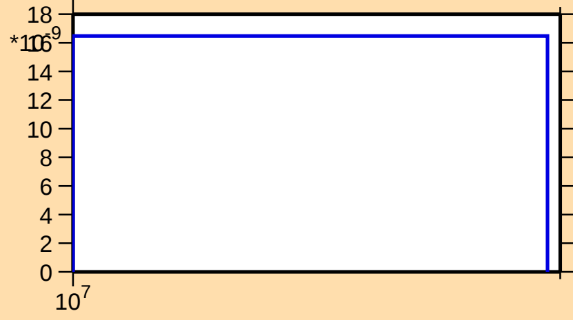
\sigma vs. E for ^{107}\text{Tc}(n,\text{nt})
