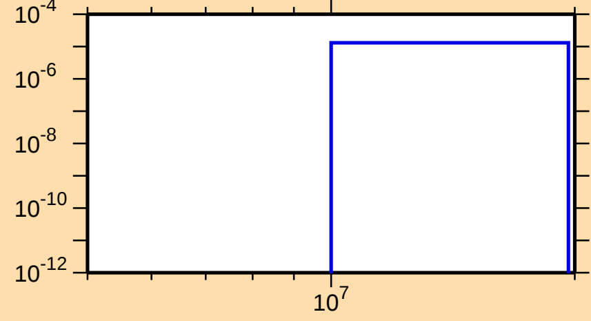
\sigma vs. E for ^{107}\text{Tc}(n,t)
