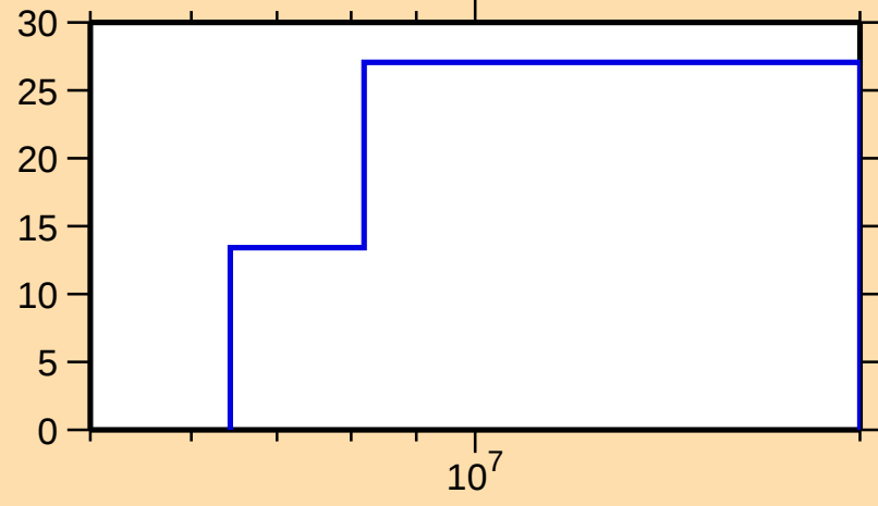
\Delta\sigma/\sigma vs. E for ^{107}\text{Tc}(n,\text{el.})
