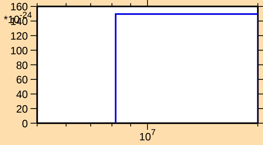
\sigma vs. E for ^{107}\text{Tc}(n,3n\alpha)
