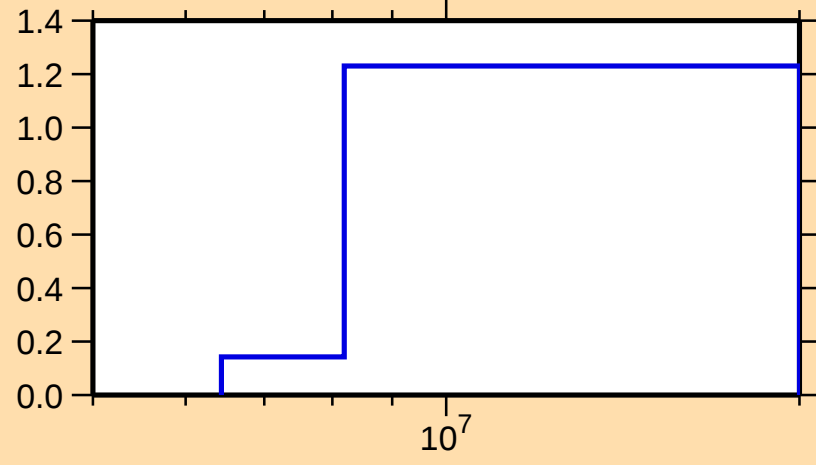
\sigma vs. E for ^{107}\text{Tc}(n,2n)
