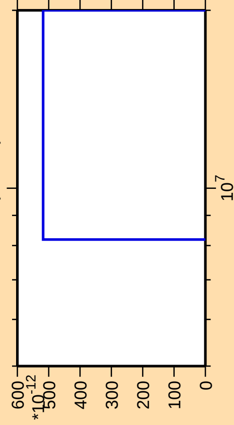
\Delta\sigma/\sigma vs. E for ^{107}\text{Tc}(\text{mt } 11)
