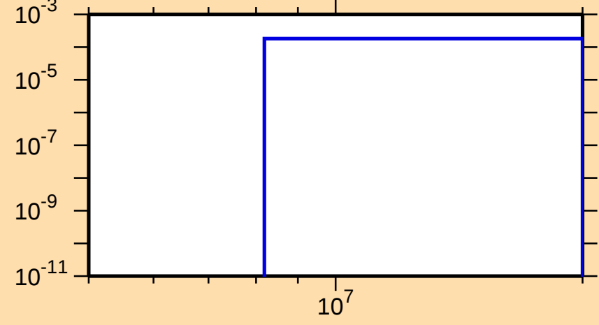
\sigma vs. E for ^{107}\text{Tc}(n,d)
