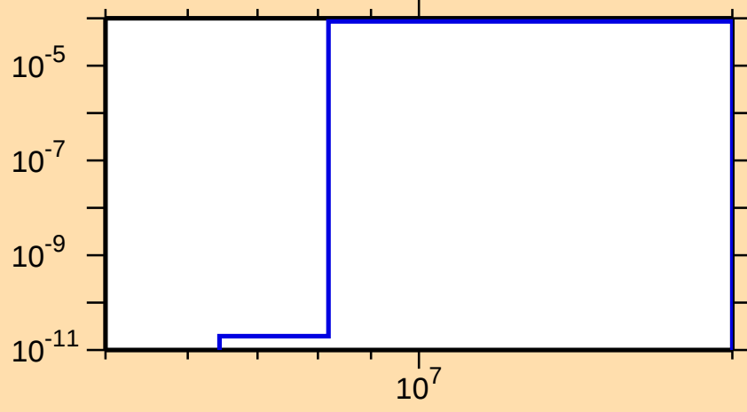
\sigma vs. E for ^{107}\text{Tc}(n,\alpha)
