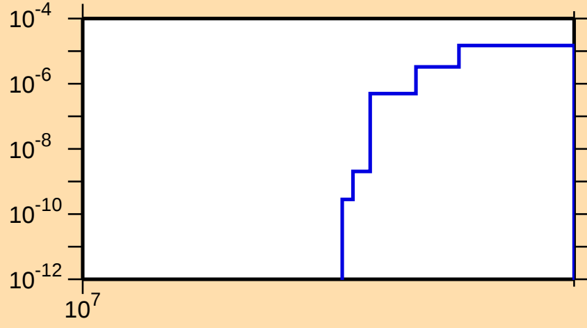
\sigma vs. E for ^{108}\text{Te}(n,2n\alpha)
