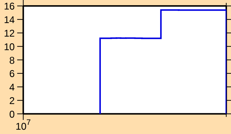
\Delta\sigma/\sigma vs. E for ^{108}\text{Te}(n,\text{el.})
