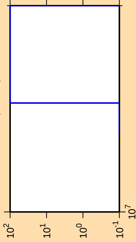
\Delta\sigma/\sigma vs. E for ^{108}\text{Te}(n,2n\alpha)
