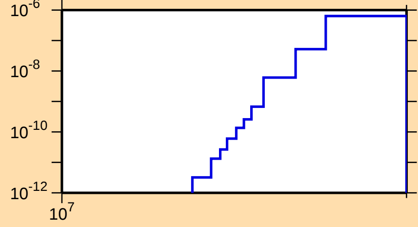
\sigma vs. E for ^{108}\text{Te}(\text{mt } 34)
