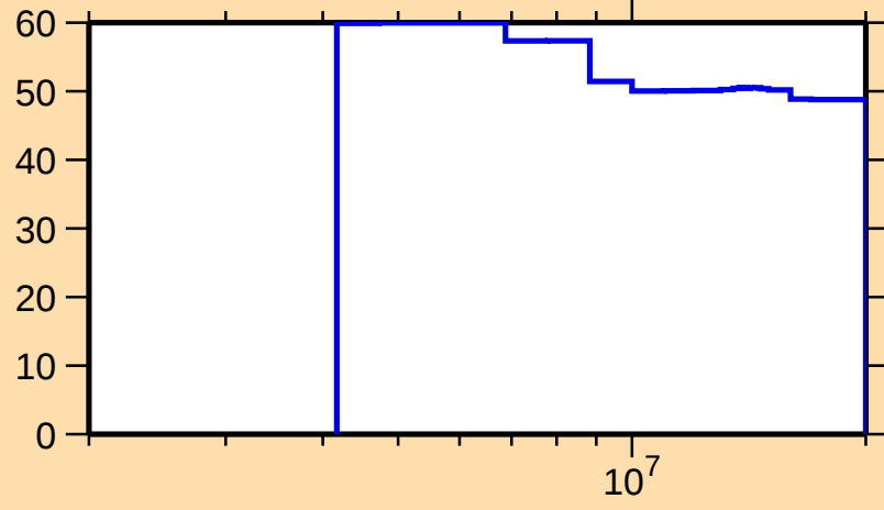
\Delta\sigma/\sigma vs. E for ^{108}\text{Te}(n,n_1)
