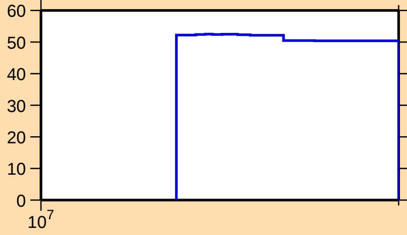
\Delta\sigma/\sigma vs. E for ^{108}\text{Te}(n,\text{inel.})
