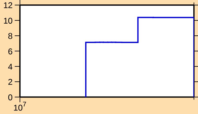
\Delta\sigma/\sigma vs. E for ^{108}\text{Te}(n,\text{tot.})
