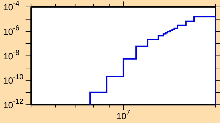
\sigma vs. E for ^{108}\text{Te}(\text{mt117})
