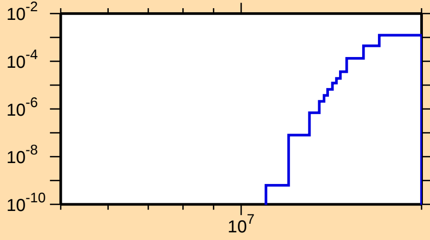
\sigma vs. E for ^{108}\text{Te}(n,\text{pt})
