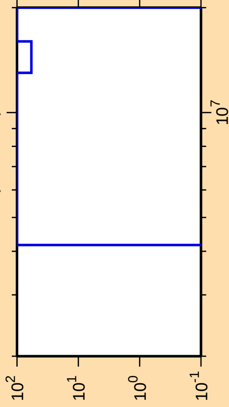
\Delta\sigma/\sigma vs. E for ^{108}\text{Te}(\text{n},\text{ncont.})
