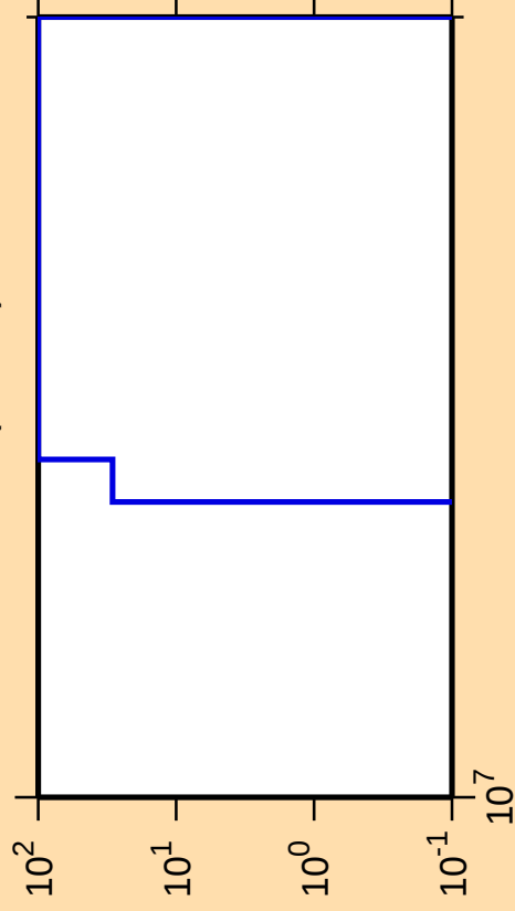
\Delta\sigma/\sigma vs. E for ^{108}\text{Te}(\text{mt } 34)
