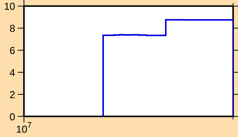
\Delta\sigma/\sigma vs. E for ^{108}\text{Te}(n,\text{nonel.})
