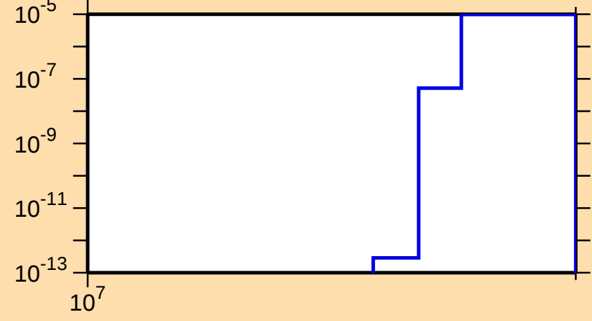
\sigma vs. E for ^{108}\text{Te}(n,2np)
