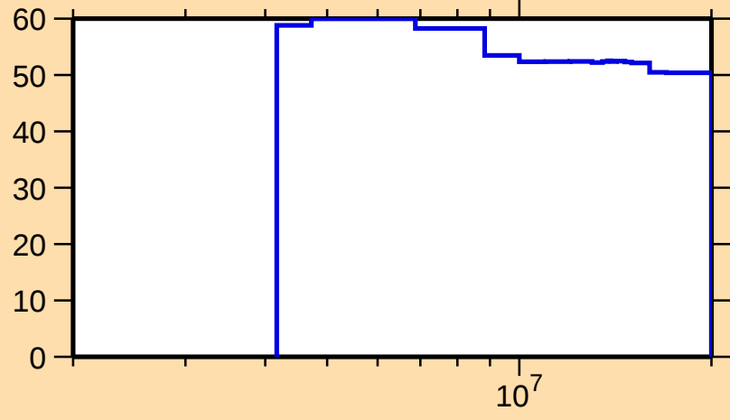
\Delta\sigma/\sigma vs. E for ^{108}\text{Te}(\text{n},\text{inel.})
