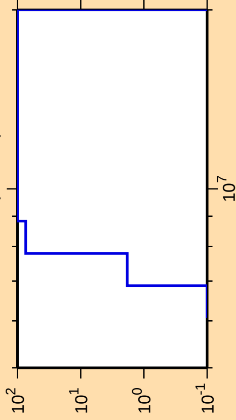
\Delta\sigma/\sigma vs. E for ^{108}\text{Te}(\text{mt117})
