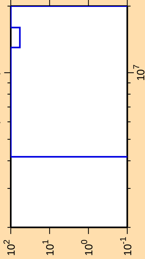
\Delta\sigma/\sigma vs. E for ^{108}\text{Te}(n,\text{ncont.})
