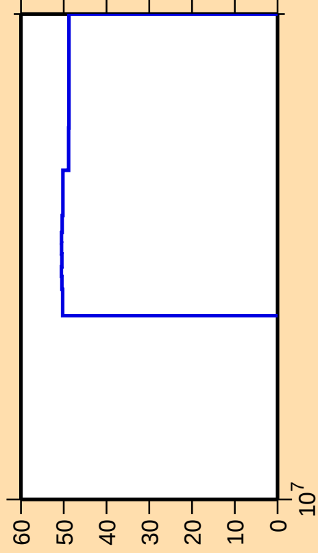
\Delta\sigma/\sigma vs. E for ^{108}\text{Te}(n,n_1)
