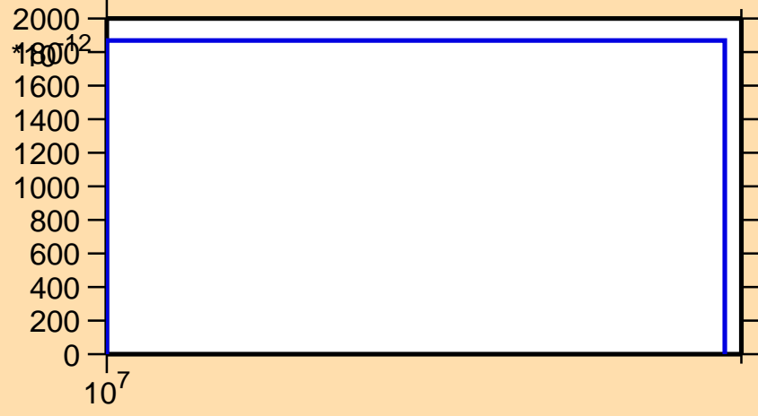
\sigma vs. E for ^{108}\text{Te}(n,nd)
