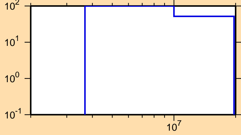
\Delta\sigma/\sigma vs. E for ^{108}\text{Te}(n,ncont.)
