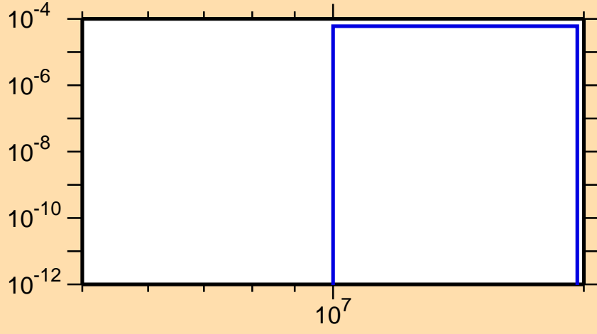
\sigma vs. E for ^{108}\text{Te}(n,\text{pt})
