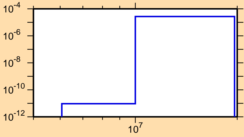
\sigma vs. E for ^{108}\text{Te}(\text{mt } 45)
