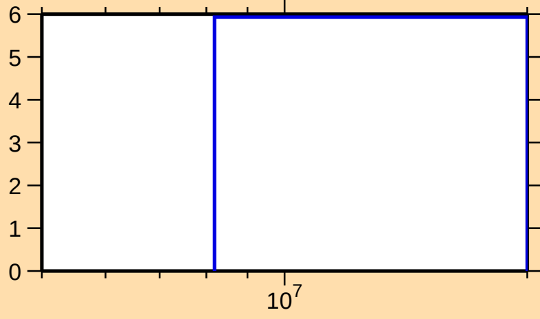
\Delta\sigma/\sigma vs. E for ^{108}\text{Te}(n,\text{tot.})
