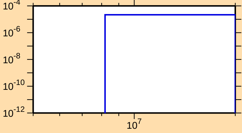
\sigma vs. E for ^{108}\text{Te}(\text{mt } 45)
