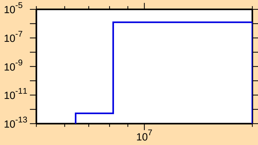
\sigma vs. E for ^{108}\text{Te}(\text{mt117})
