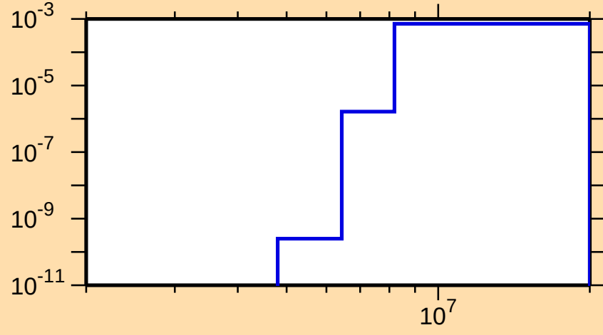
\sigma vs. E for ^{108}\text{Te}(n,n\text{cont.})
