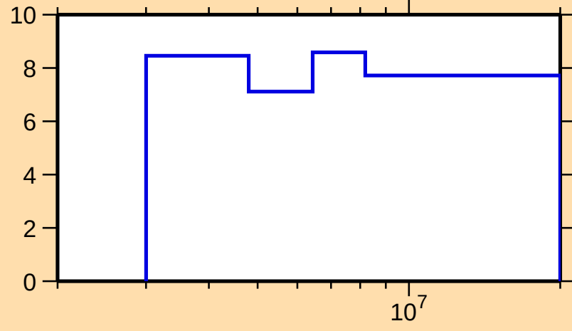
\Delta\sigma/\sigma vs. E for ^{108}\text{Te}(n,n\text{onel.})
