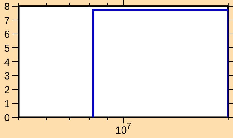
\Delta\sigma/\sigma vs. E for ^{108}\text{Te}(n,\text{nonel.})
