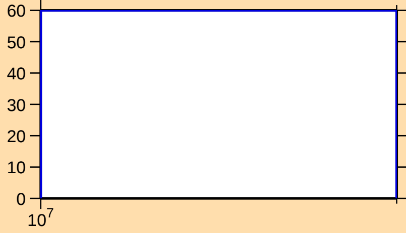
\Delta\sigma/\sigma vs. E for ^{109}\text{Te}(n,2n)
