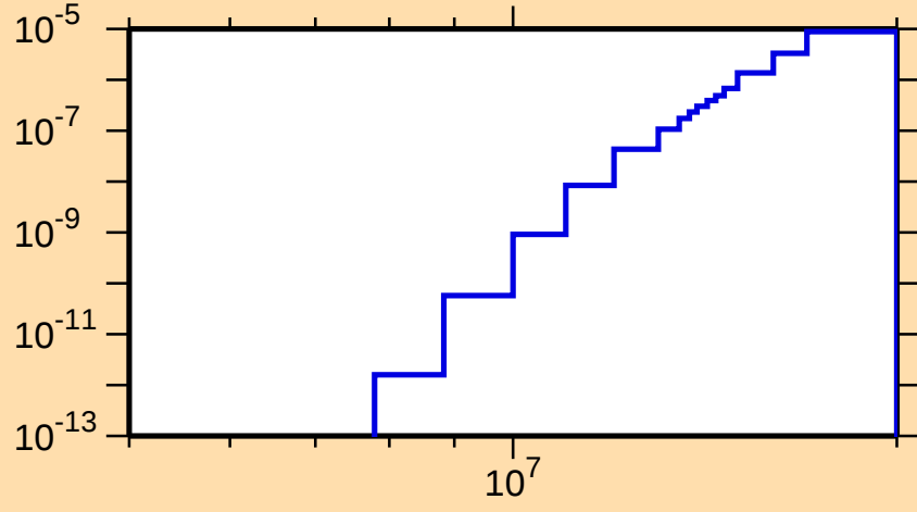
\sigma vs. E for ^{109}\text{Te}(\text{mt117})
