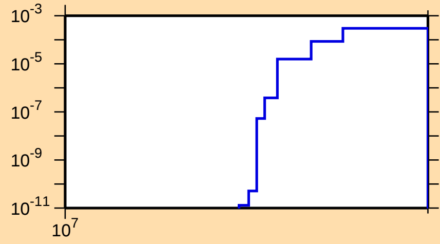
\sigma vs. E for ^{109}\text{Te}(n,2np)
