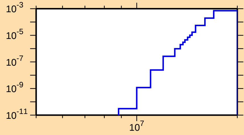
\sigma vs. E for ^{109}\text{Te}(\text{mt } 45)
