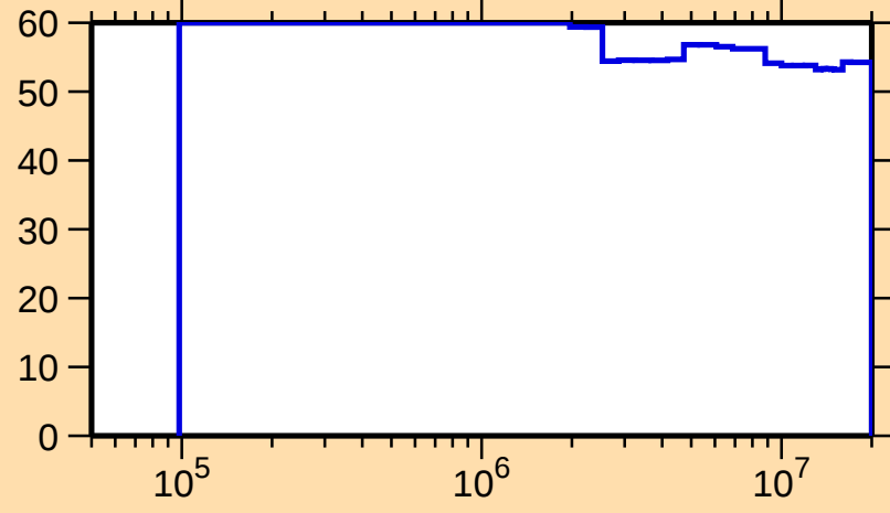
\Delta\sigma/\sigma vs. E for ^{109}\text{Te}(n,\text{inel.})
