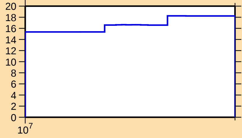
\Delta\sigma/\sigma vs. E for ^{109}\text{Te}(n,\text{nonel.})
