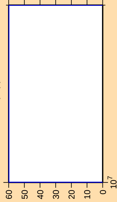
\Delta\sigma/\sigma vs. E for ^{109}\text{Te}(n,p)
