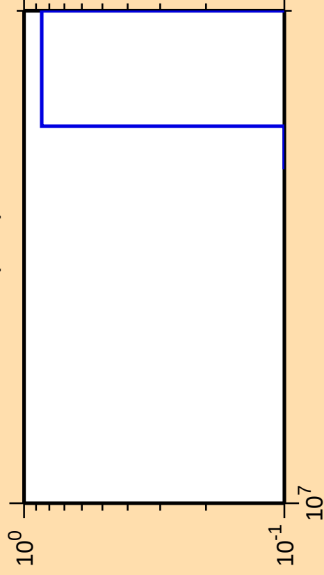
\Delta\sigma/\sigma vs. E for ^{109}\text{Te}(n,\text{nt})
