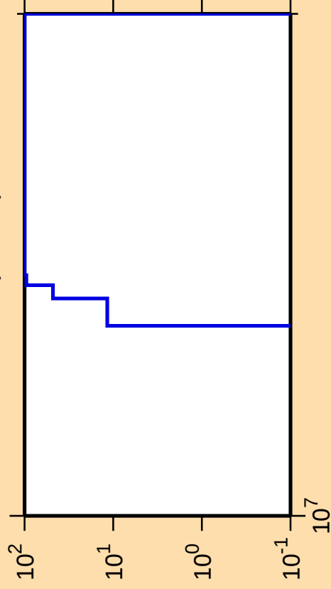
\Delta\sigma/\sigma vs. E for ^{109}\text{Te}(n,2n\alpha)
