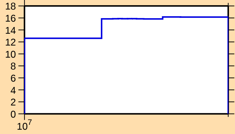
\Delta\sigma/\sigma vs. E for ^{109}\text{Te}(n,\text{tot.})
