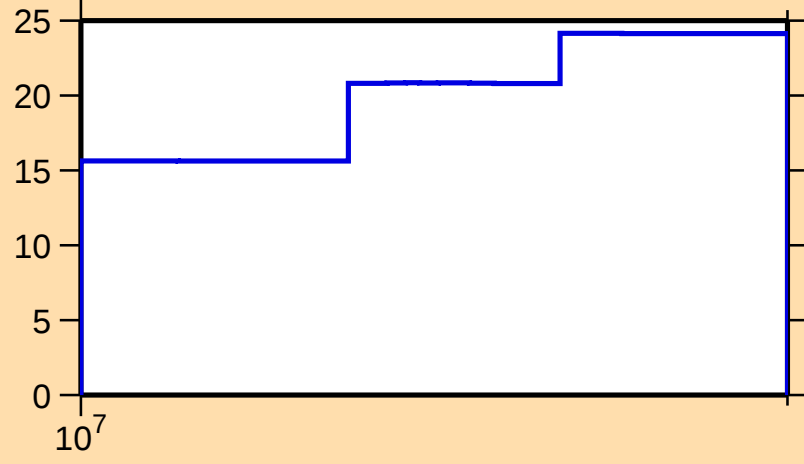
\Delta\sigma/\sigma vs. E for ^{109}\text{Te}(n,\text{el.})
