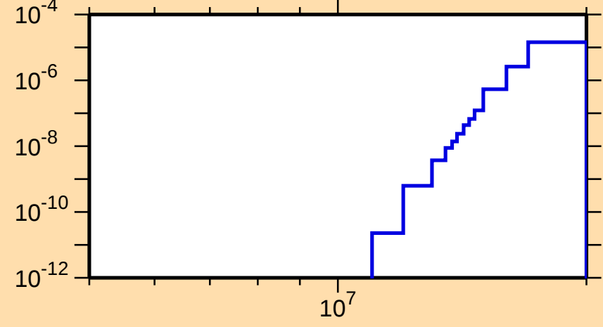
\sigma vs. E for ^{109}\text{Te}(\text{mt } 34)
