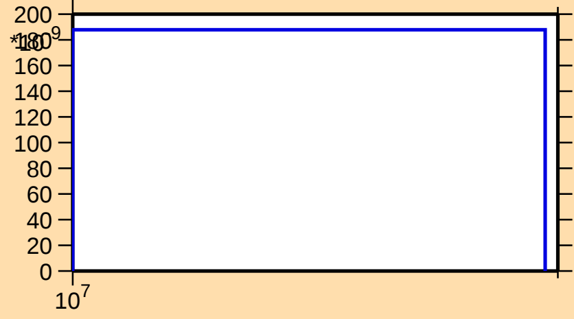
\sigma vs. E for ^{109}\text{Te}(n,\text{nd})
