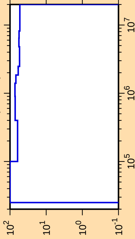
\Delta\sigma/\sigma vs. E for ^{109}\text{Te}(n,\text{inel.})
