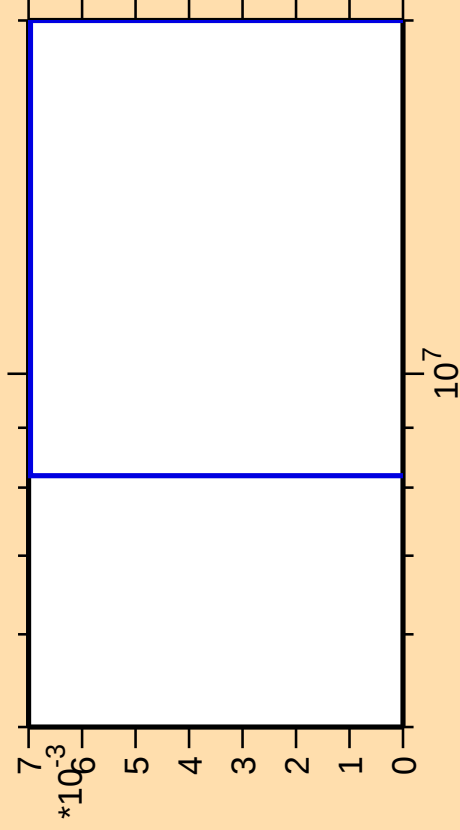
\Delta\sigma/\sigma vs. E for ^{109}\text{Te}(n,nt)
