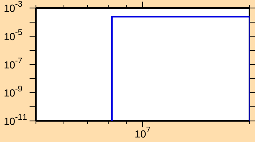
\sigma vs. E for ^{109}\text{Te}(n,\text{pt})
