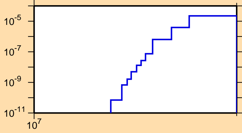
\sigma vs. E for ^{111}\text{Te}(n,nd)
