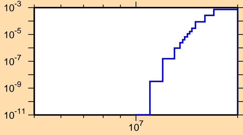
\sigma vs. E for ^{111}\text{Te}(n,\text{pt})
