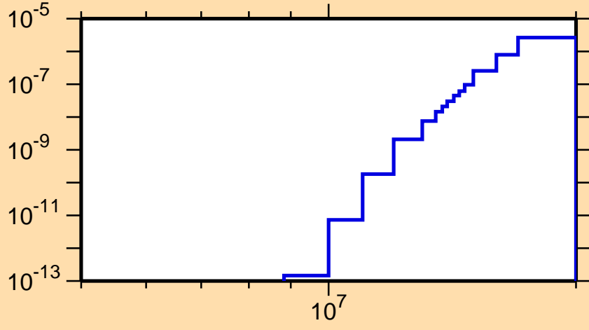
\sigma vs. E for ^{111}\text{Te}(\text{mt117})
