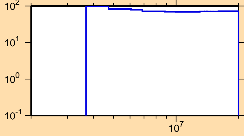
\Delta\sigma/\sigma vs. E for ^{111}\text{Te}(n,n\text{cont.})
