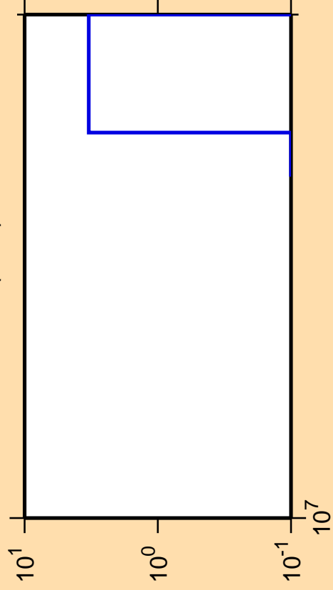
\Delta\sigma/\sigma vs. E for ^{111}\text{Te}(n,nt)
