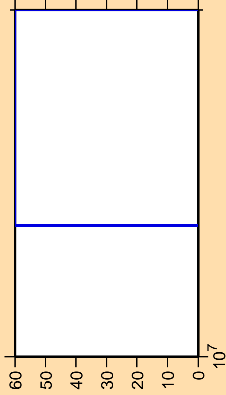
\Delta\sigma/\sigma vs. E for ^{111}\text{Te}(n,nd)
