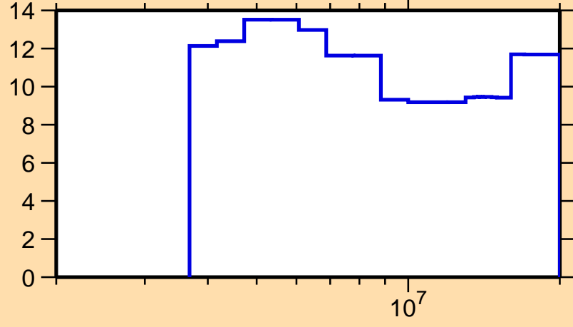
\Delta\sigma/\sigma vs. E for ^{111}\text{Te}(n,n\text{onel.})
