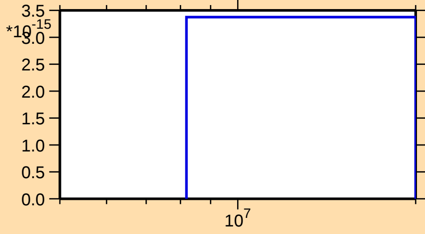
\sigma vs. E for ^{111}\text{Te}(n,nt)
