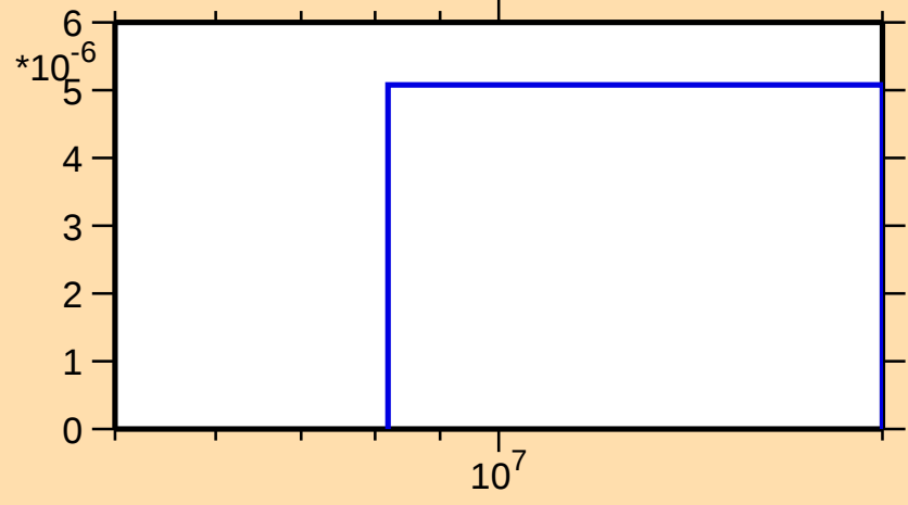
\sigma vs. E for ^{111}\text{Te}(\text{mt } 45)
