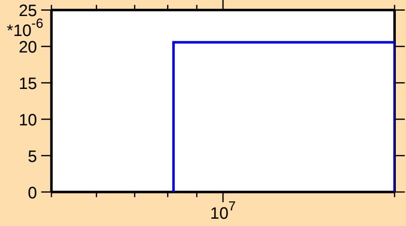
\sigma vs. E for ^{111}\text{Te}(n,2np)
