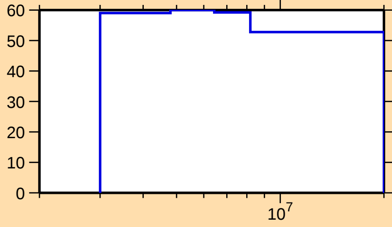
\Delta\sigma/\sigma vs. E for ^{111}\text{Te}(n,\text{inel.})
