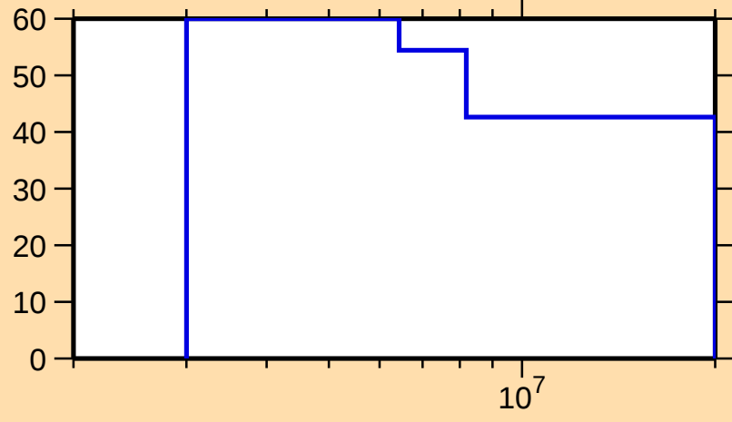
\Delta\sigma/\sigma vs. E for ^{111}\text{Te}(n, n_1)
