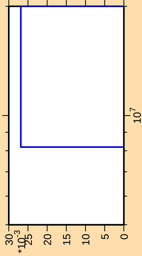
\Delta\sigma/\sigma vs. E for ^{111}\text{Te}(n,nt)
