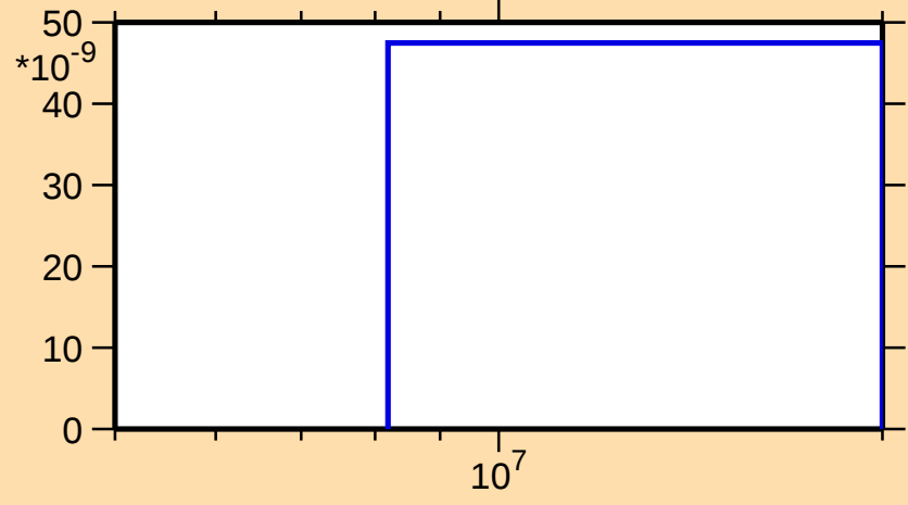
\sigma vs. E for ^{111}\text{Te}(\text{mt } 34)
