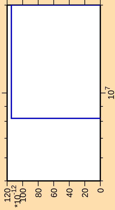
\Delta\sigma/\sigma vs. E for ^{111}\text{Te}(n,3n\alpha)
