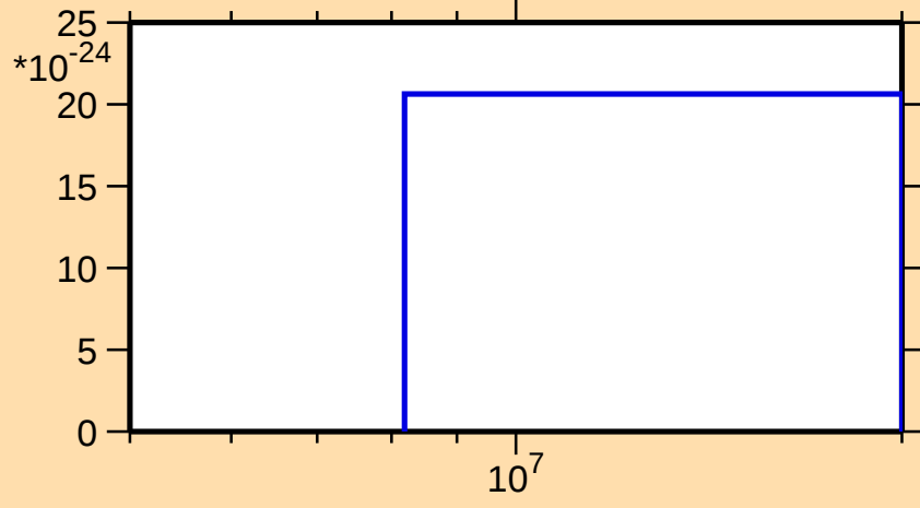
\sigma vs. E for ^{111}\text{Te}(n,3n\alpha)
