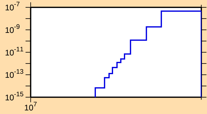
\sigma vs. E for ^{115}\text{Te}(\text{mt } 34)
