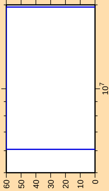
\Delta\sigma/\sigma vs. E for ^{115}\text{Te}(n,n_1)
