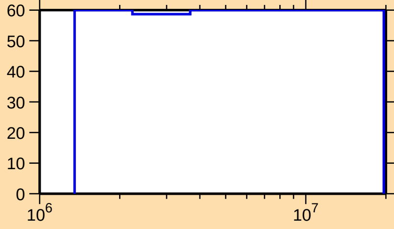
\Delta\sigma/\sigma vs. E for ^{115}\text{Te}(n,n_1)
