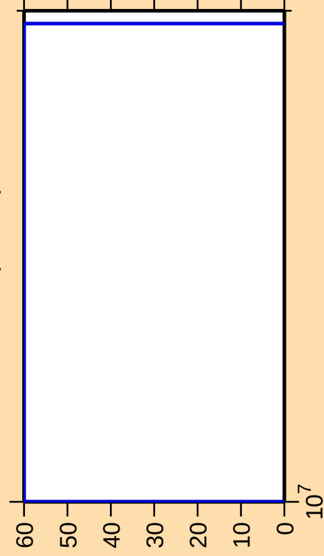
\Delta\sigma/\sigma vs. E for ^{115}\text{Te}(\text{mt } 34)
