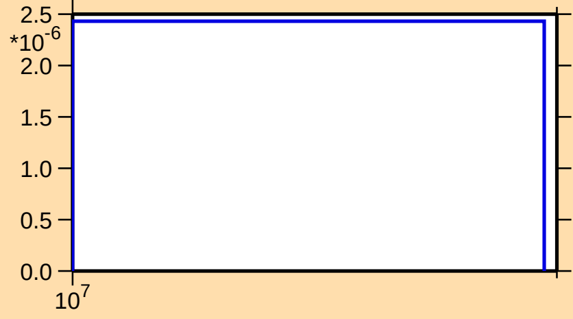
\sigma vs. E for ^{115}\text{Te}(n,\text{nd})
