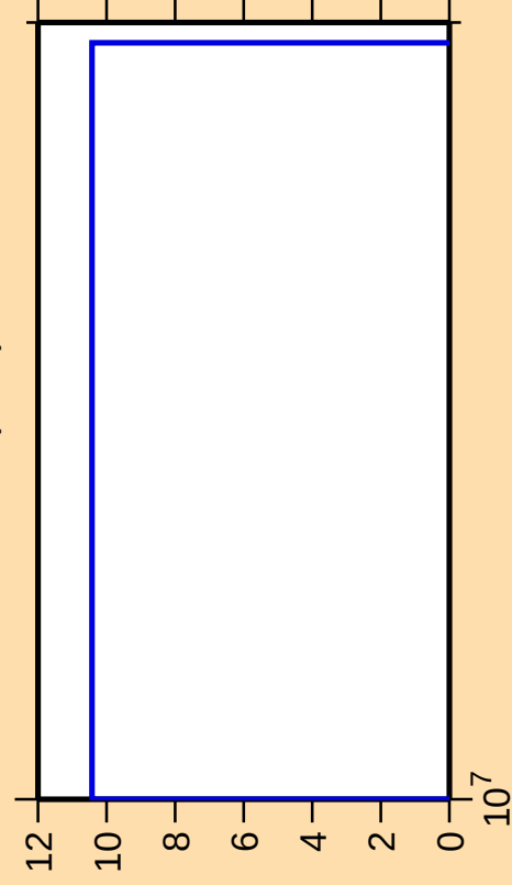
\Delta\sigma/\sigma vs. E for ^{115}\text{Te}(n,\text{nt})
