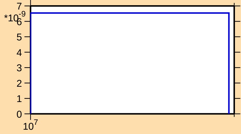
\sigma vs. E for ^{115}\text{Te}(\text{mt } 45)
