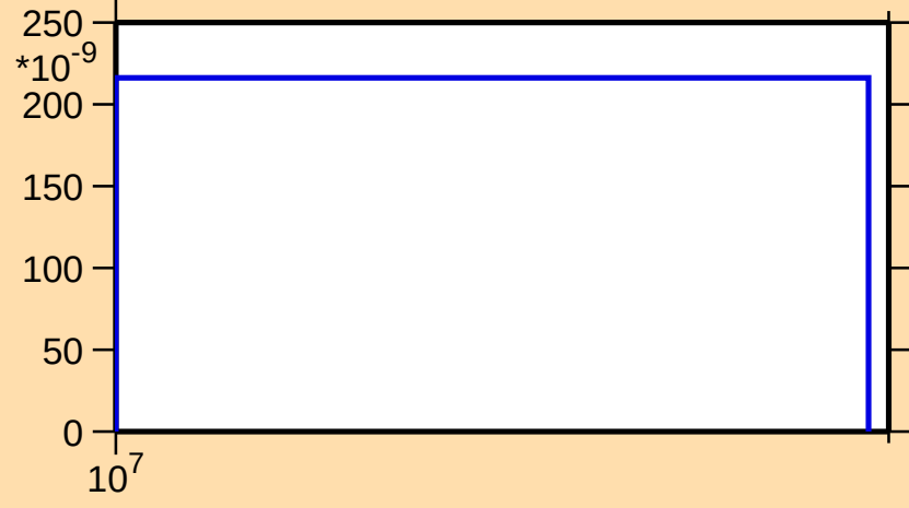
\sigma vs. E for ^{115}\text{Te}(n,\text{pt})
