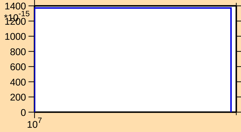
\sigma vs. E for ^{115}\text{Te}(n,\text{nt})
