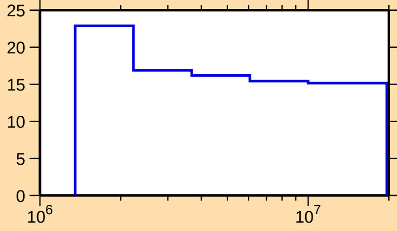
\Delta\sigma/\sigma vs. E for ^{115}\text{Te}(n,n\text{onel.})
