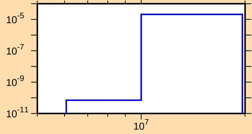
\sigma vs. E for ^{115}\text{Te}(n,\text{He3})
