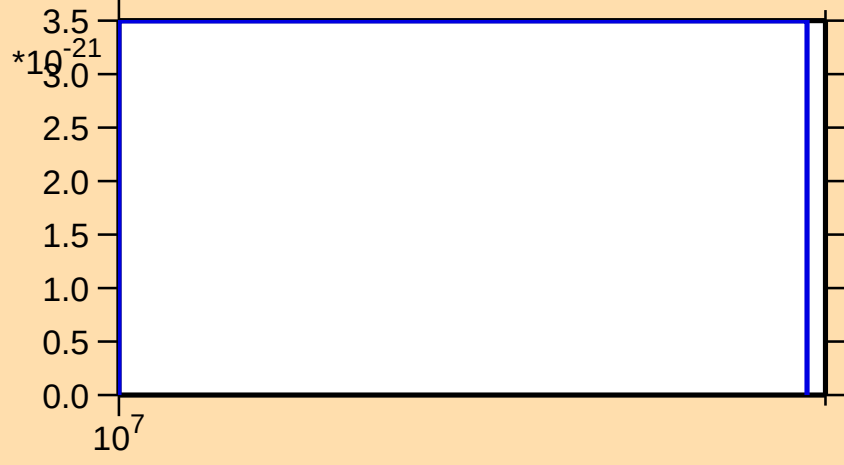
\sigma vs. E for ^{115}\text{Te}(n,3n\alpha)
