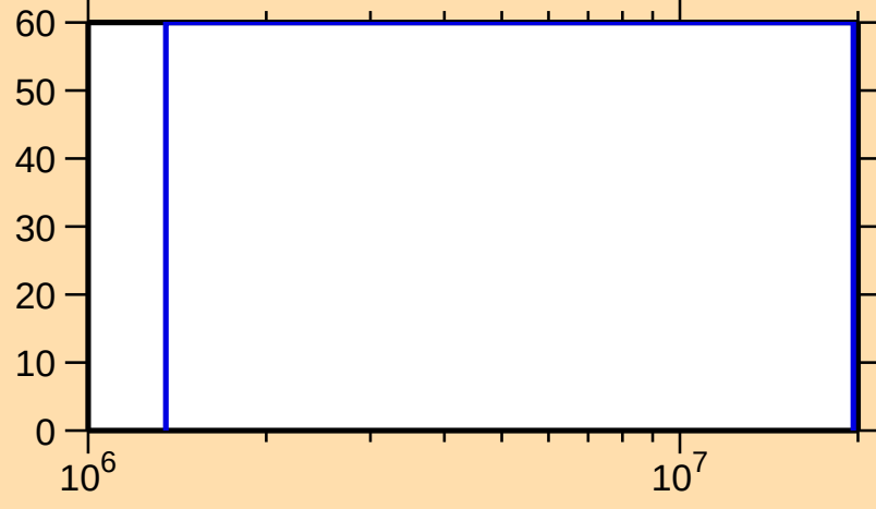
\Delta\sigma/\sigma vs. E for ^{115}\text{Te}(n,n\text{cont.})
