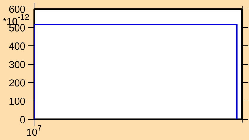
\sigma vs. E for ^{115}\text{Te}(\text{mt } 34)
