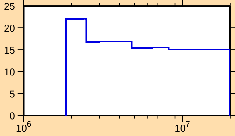
\Delta\sigma/\sigma vs. E for ^{115}\text{Te}(n,n\text{oncl.})
