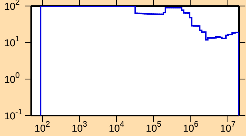
\Delta\sigma/\sigma vs. E for ^{115}\text{Te}(n,\text{nonel.})
