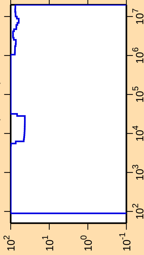
\Delta\sigma/\sigma vs. E for ^{115}\text{Te}(n,\text{inel.})
