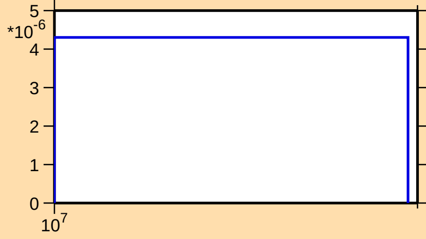
\sigma vs. E for ^{115}\text{Te}(n,\text{nd})
