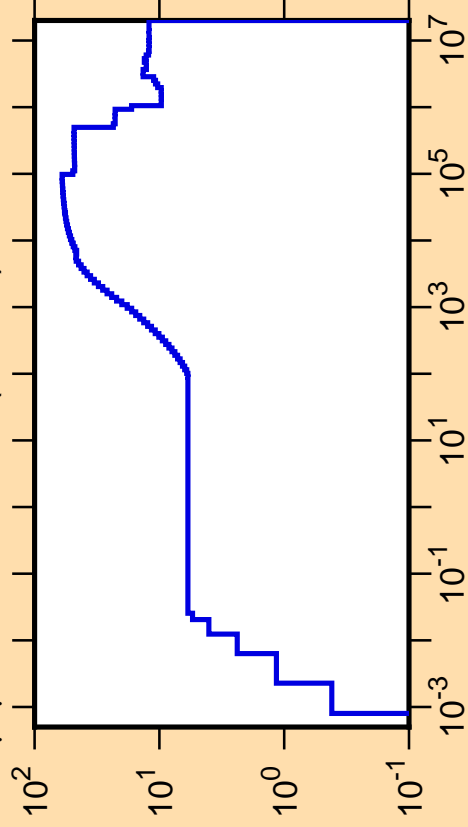
\Delta\mu/\mu vs. E for ^{117}\text{Te}(\text{mt251})
