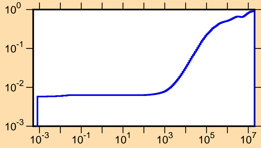
\mu vs. E for ^{117}\text{Te}(\text{mt251})
