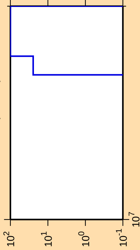
\Delta\sigma/\sigma vs. E for ^{117}\text{Te}(\text{mt117})
