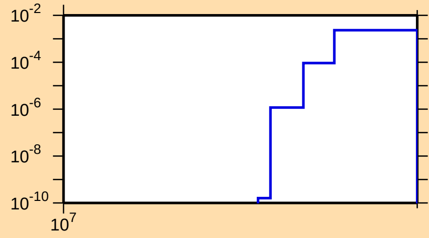
\sigma vs. E for ^{117}\text{Te}(n,2np)
