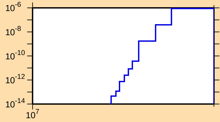
\sigma vs. E for ^{117}\text{Te}(n,\text{pt})
