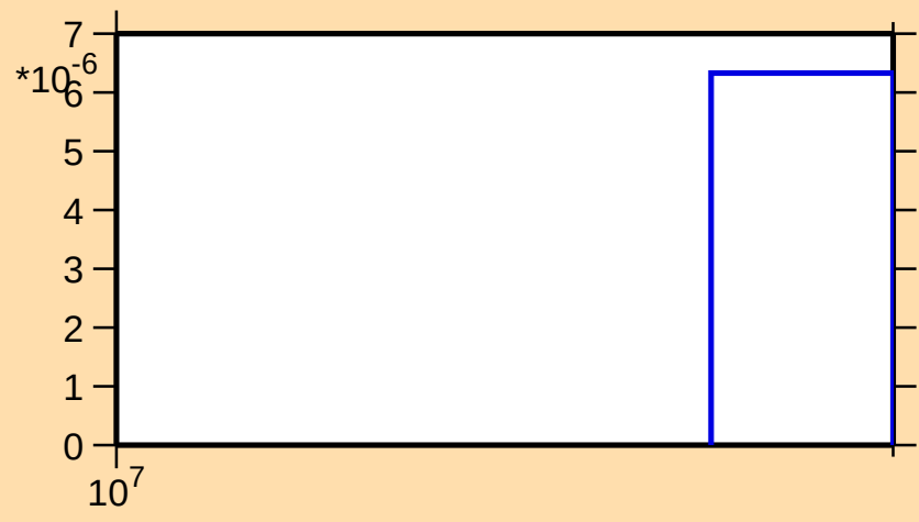
\sigma vs. E for ^{117}\text{Te}(n,3n)
