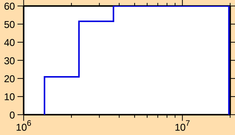
\Delta\sigma/\sigma vs. E for ^{117}\text{Te}(n, n_1)
