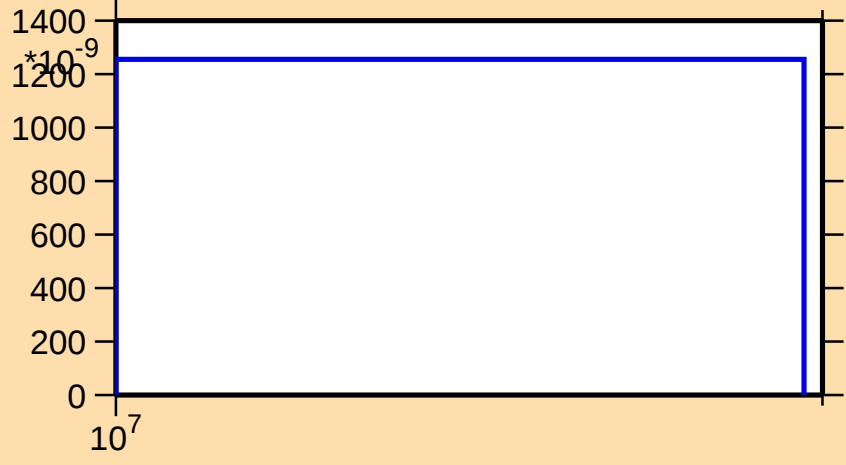
\sigma vs. E for ^{117}\text{Te}(n,\text{nd})
