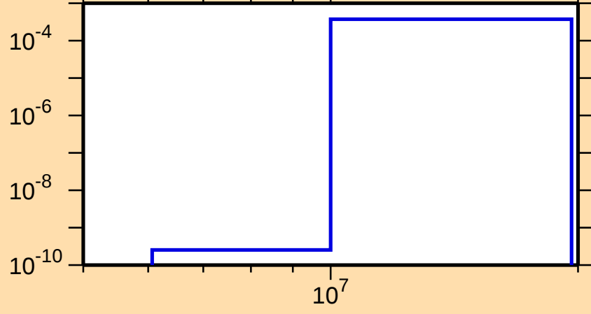
\sigma vs. E for ^{117}\text{Te}(n,t)
