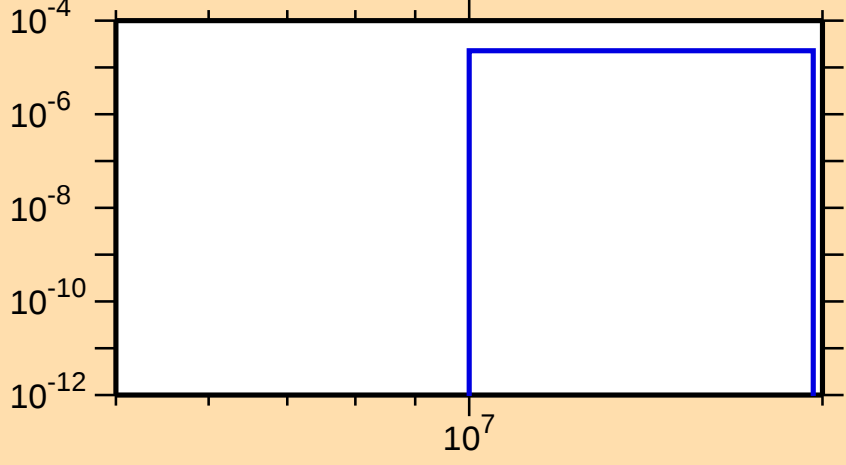
\sigma vs. E for ^{117}\text{Te}(n,2n\alpha)
