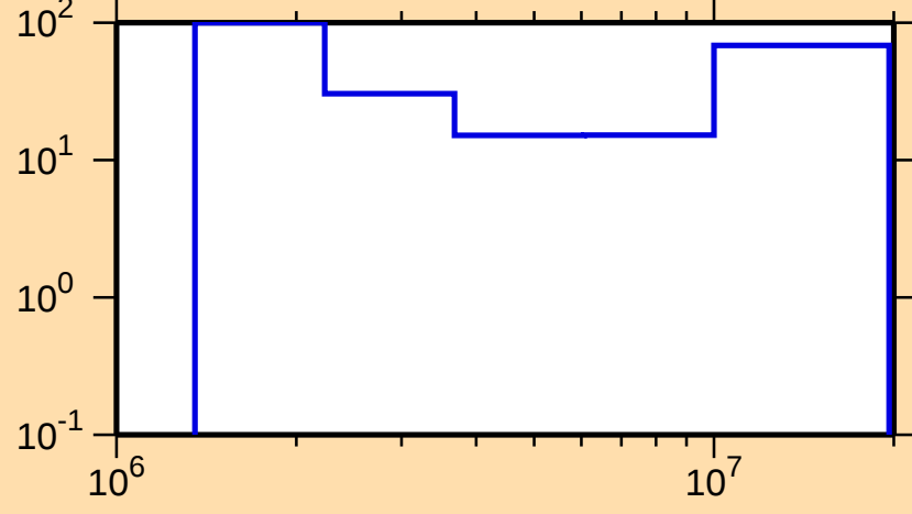
\Delta\sigma/\sigma vs. E for ^{117}\text{Te}(n,n\text{cont.})
