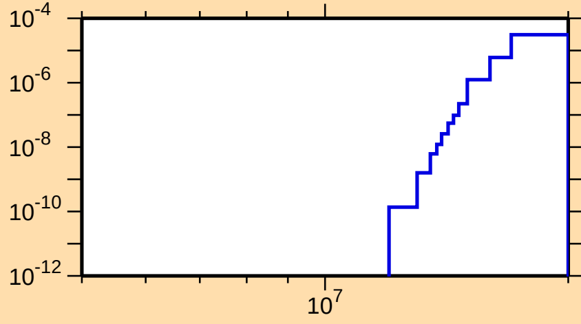
\sigma vs. E for ^{119}\text{Te}(n,2n\alpha)
