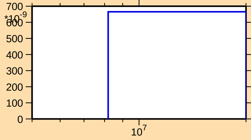
\sigma vs. E for ^{119}\text{Te}(n,2n\alpha)
