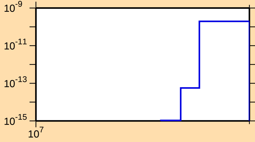
\sigma vs. E for ^{120}\text{Te}(n,\text{nt})
