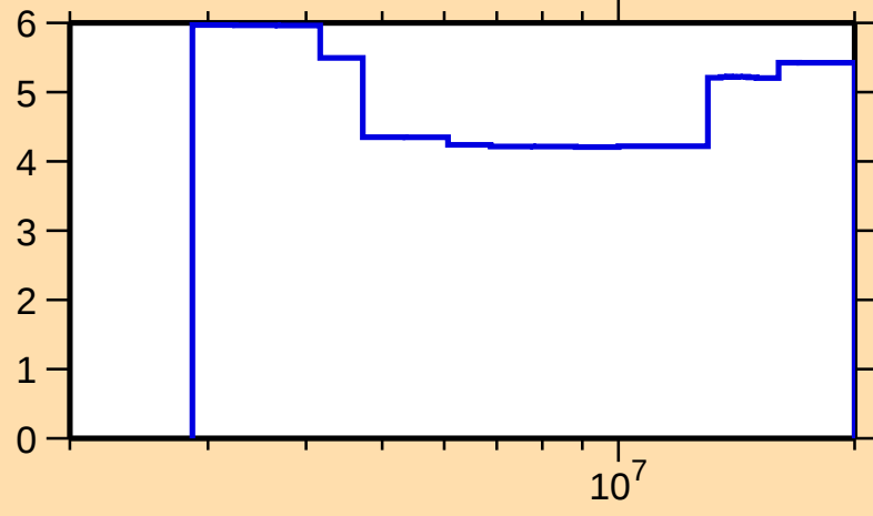
\Delta\sigma/\sigma vs. E for ^{120}\text{Te}(n,n\text{oncl.})
