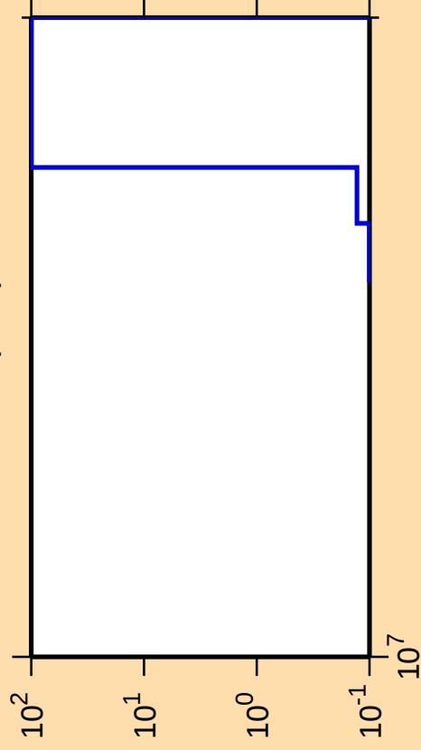
\Delta\sigma/\sigma vs. E for ^{120}\text{Te}(n,\text{nt})
