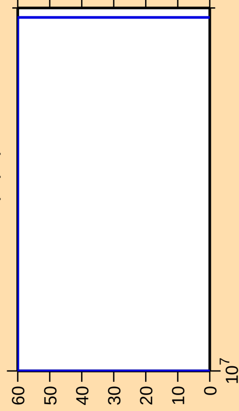
\Delta\sigma/\sigma vs. E for ^{120}\text{Te}(n,\text{pd})
