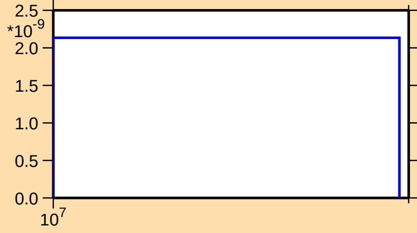
\sigma vs. E for ^{120}\text{Te}(n,2n\alpha)
