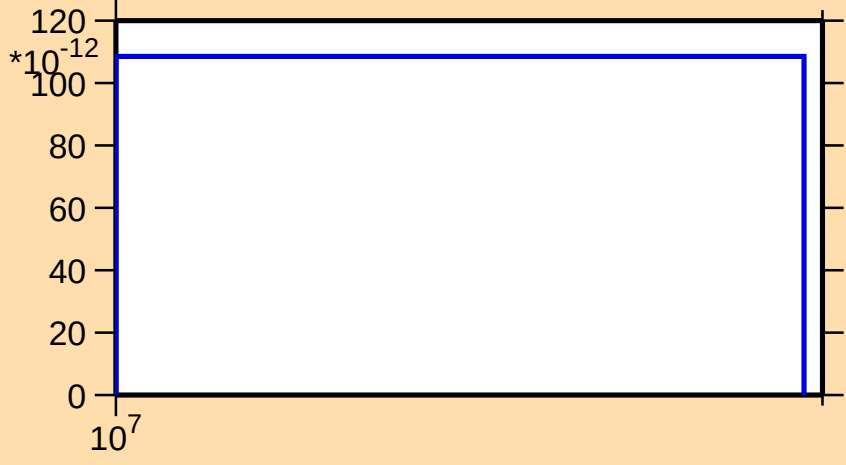
\sigma vs. E for ^{120}\text{Te}(n,\text{pd})
