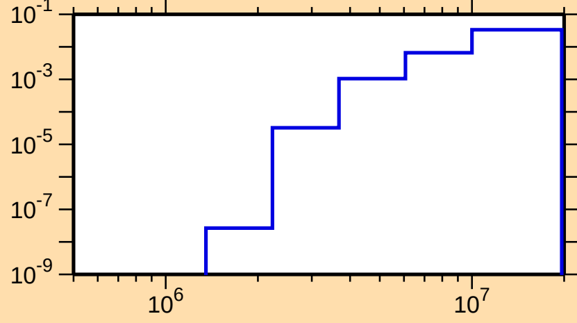
\sigma vs. E for ^{120}\text{Te}(n,p)
