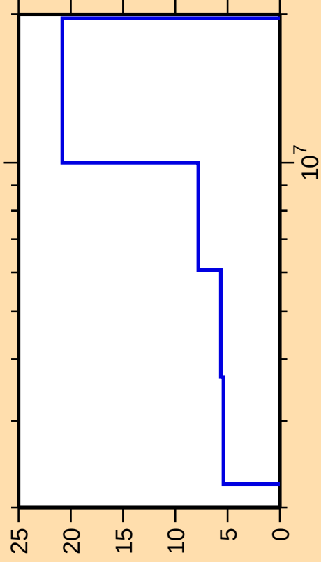
\Delta\sigma/\sigma vs. E for ^{120}\text{Te}(n,\text{ncont.})
