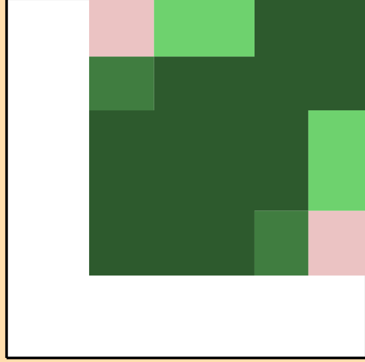
\sigma vs. E for ^{121}\text{Te}(n,2n)
