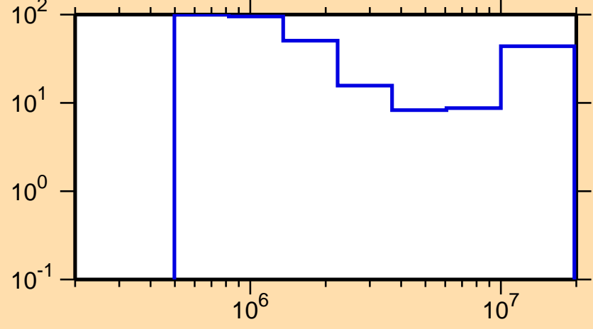
\Delta\sigma/\sigma vs. E for ^{121}\text{Te}(n,n\text{cont.})
