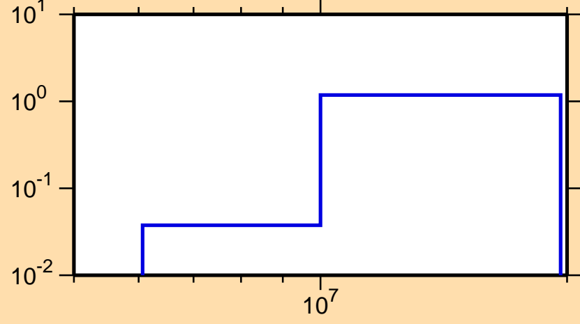
\sigma vs. E for ^{121}\text{Te}(n,2n)
