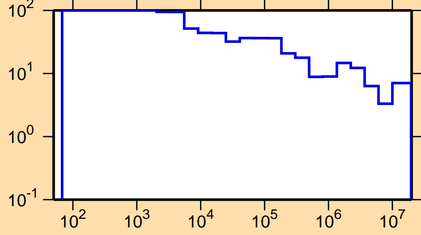
\Delta\sigma/\sigma vs. E for ^{121}\text{Te}(n,\text{tot.})
