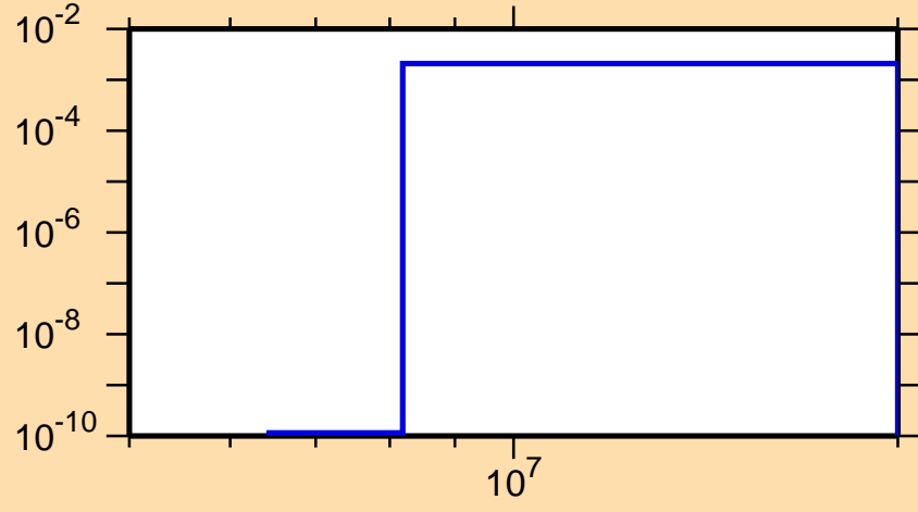
\sigma vs. E for ^{121}\text{Te}(n,d)
