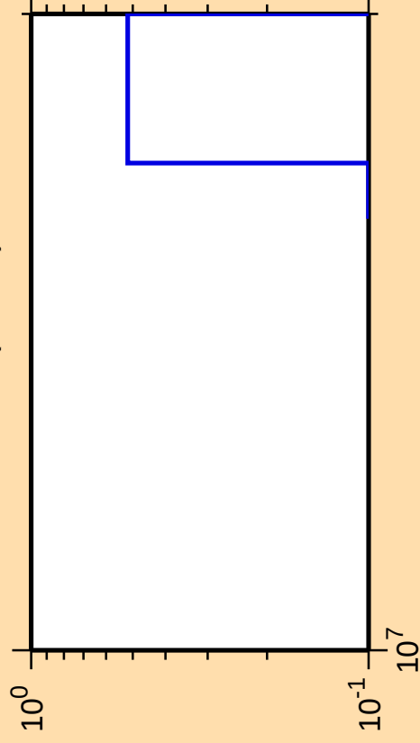
\Delta\sigma/\sigma vs. E for ^{123}\text{Te} (mt 34)
