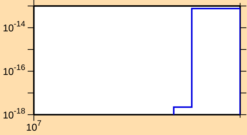
\sigma vs. E for ^{123}\text{Te} (mt 34)
