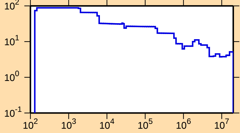
\Delta\sigma/\sigma vs. E for ^{123}\text{Te}(n,\text{tot.})
