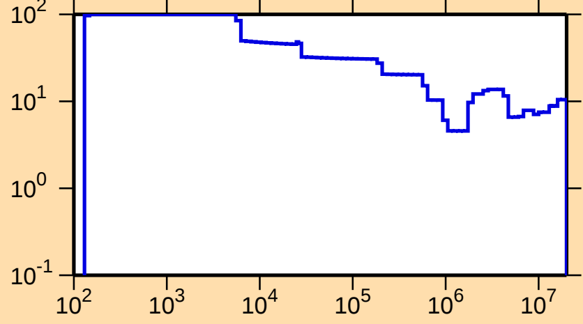
\Delta\sigma/\sigma vs. E for ^{123}\text{Te}(n,\text{el.})
