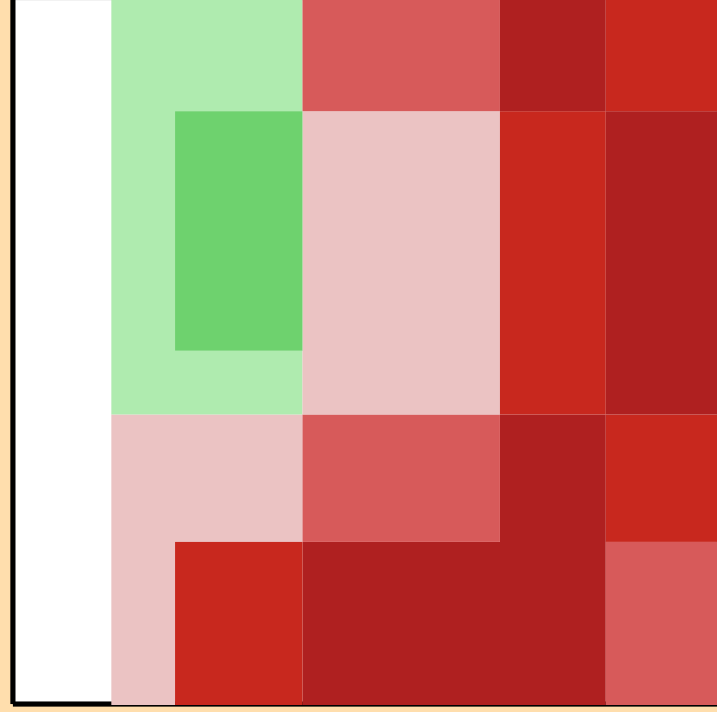
\Delta\sigma/\sigma vs. E for ^{123}\text{Te}(n,2n)
