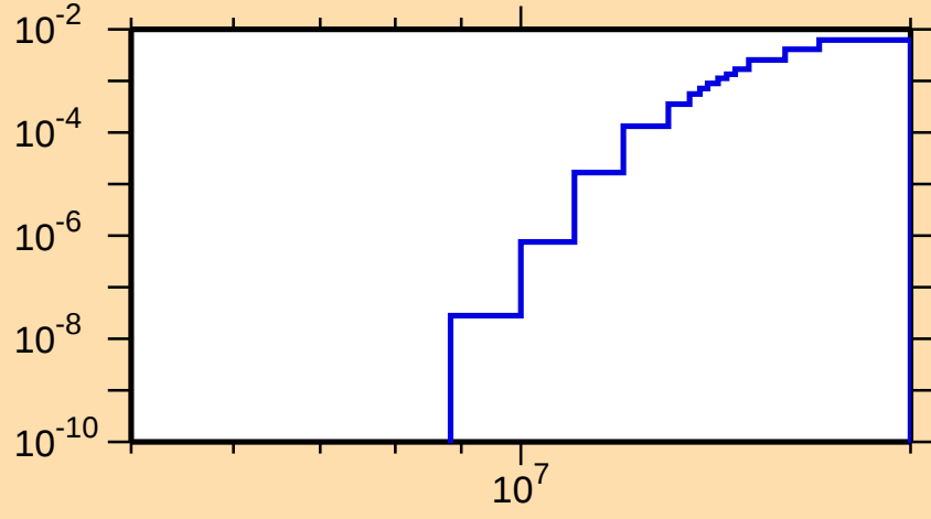
\sigma vs. E for ^{123}\text{Te}(n,d)
