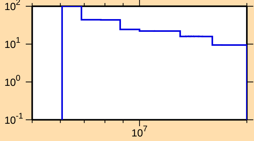
\Delta\sigma/\sigma vs. E for ^{123}\text{Te}(n,2n)
