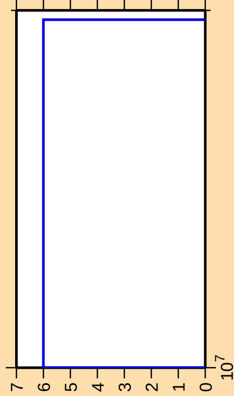
\Delta\sigma/\sigma vs. E for ^{123}\text{Te}(n,p\alpha)
