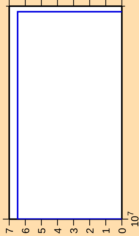
\Delta\sigma/\sigma vs. E for ^{123}\text{Te}(n,\text{nt})
