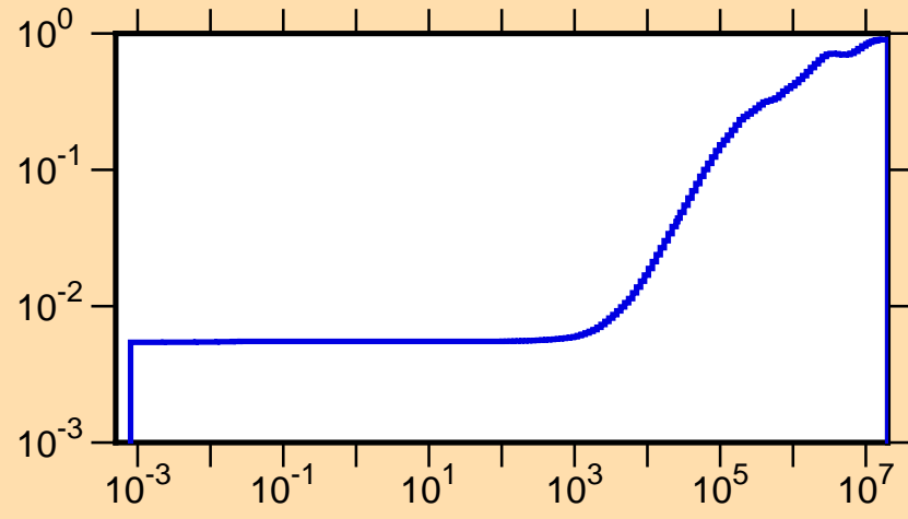
\mu vs. E for ^{124}\text{Te}(\text{mt251})
