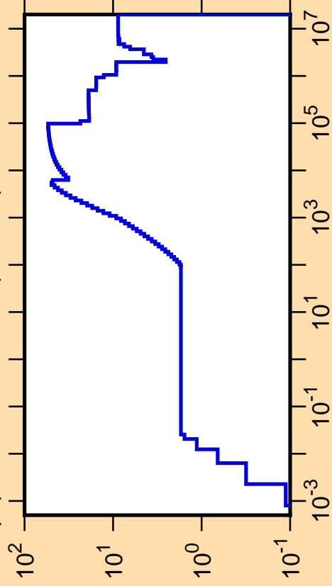
\Delta\mu/\mu vs. E for ^{124}\text{Te}(\text{mt251})
