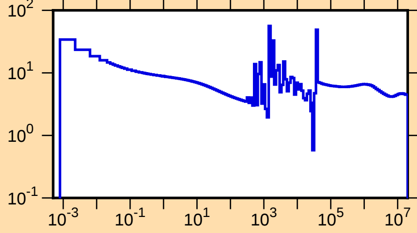
\sigma vs. E for ^{124}\text{Te}(n,\text{tot.})
