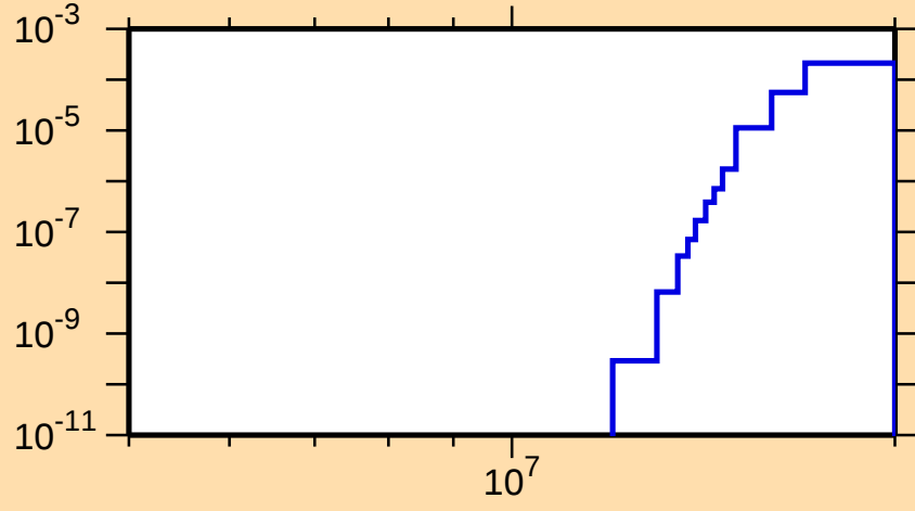
\sigma vs. E for ^{124}\text{Te}(n,t)
