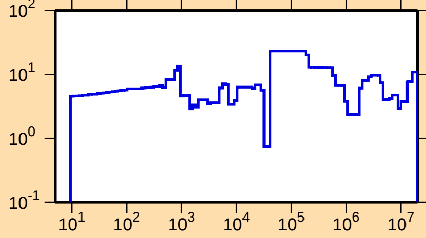
\Delta\sigma/\sigma vs. E for ^{124}\text{Te}(n,\text{el.})
