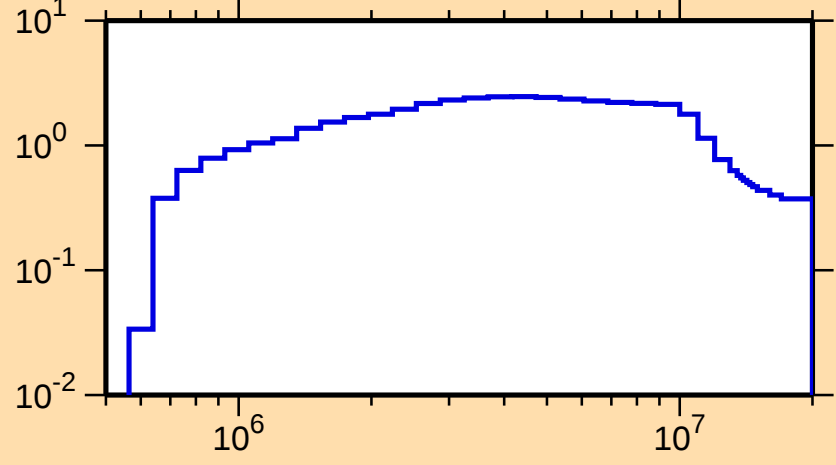
\sigma vs. E for ^{124}\text{Te}(n,\text{inel.})
