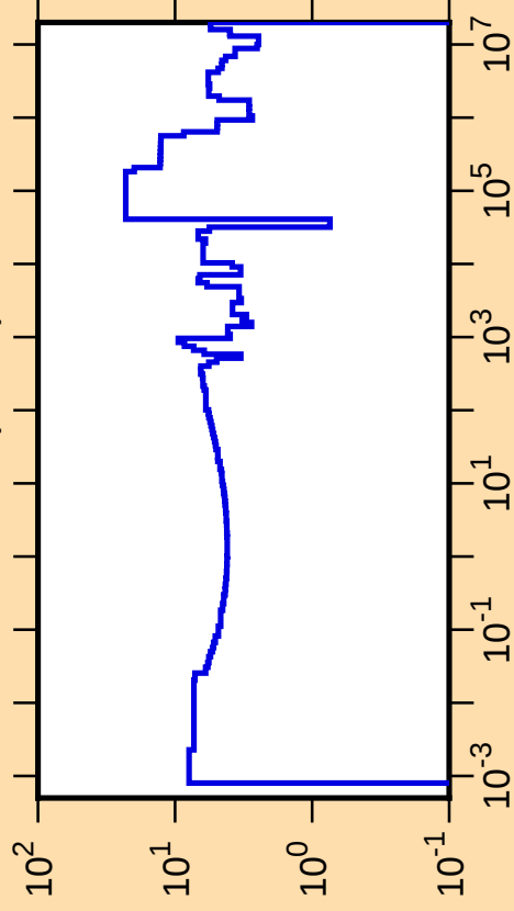
\Delta\sigma/\sigma vs. E for ^{124}\text{Te}(n,\text{tot.})
