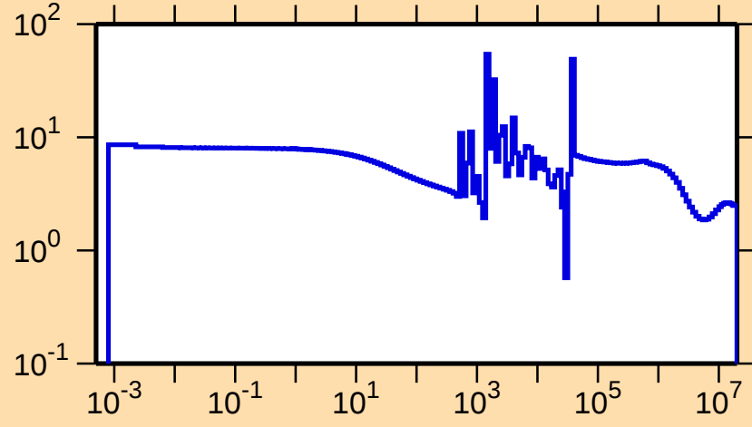
\sigma vs. E for ^{124}\text{Te}(n,\text{el.})
