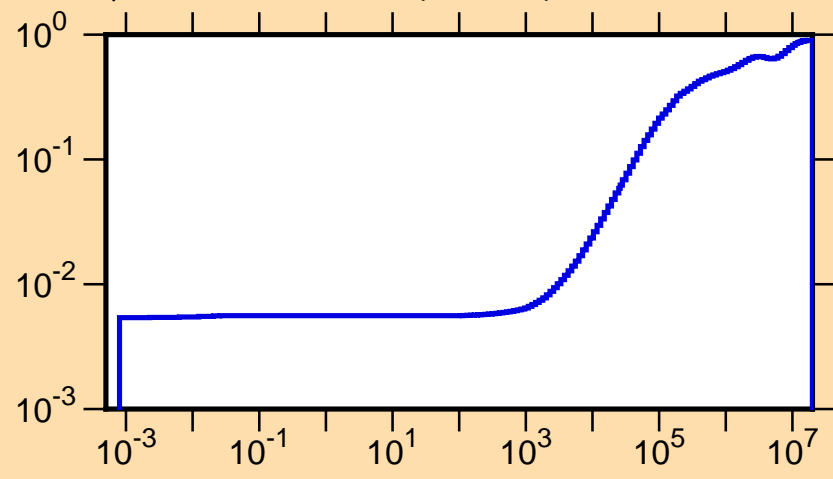
\mu vs. E for ^{125}\text{Te}(\text{mt251})
