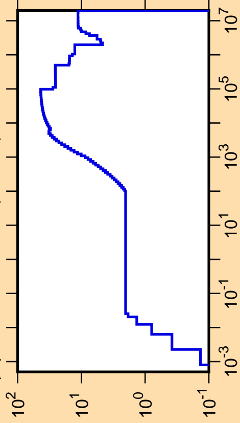
\Delta\mu/\mu vs. E for ^{125}\text{Te}(\text{mt251})
