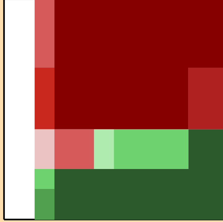
\Delta\sigma/\sigma vs. E for ^{125}\text{Te}(n,2n)
