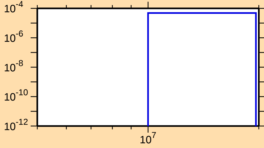
\sigma vs. E for ^{125}\text{Te}(n,t)
