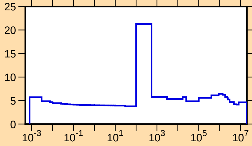
\sigma vs. E for ^{126}\text{Te}(n,\text{tot.})
