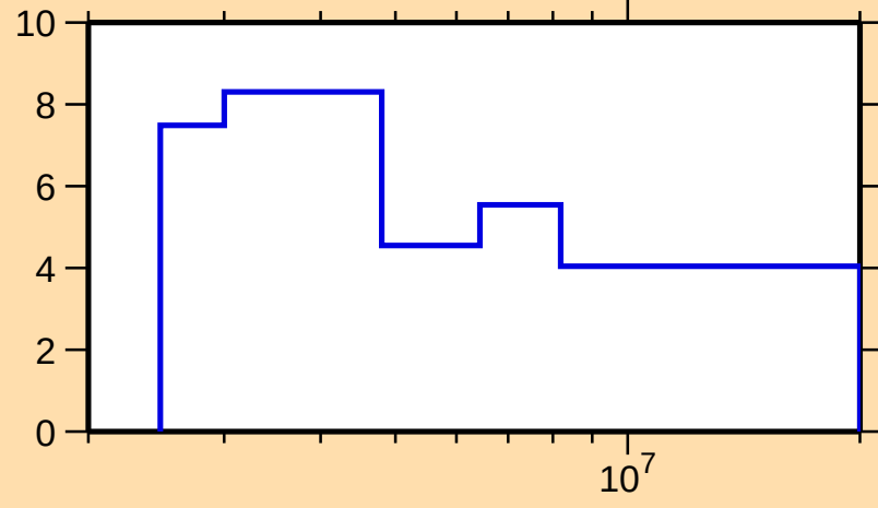
\Delta\sigma/\sigma vs. E for ^{126}\text{Te}(n,n\text{onel.})
