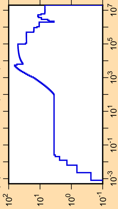
\Delta\mu/\mu vs. E for ^{127}\text{Te}(\text{mt251})
