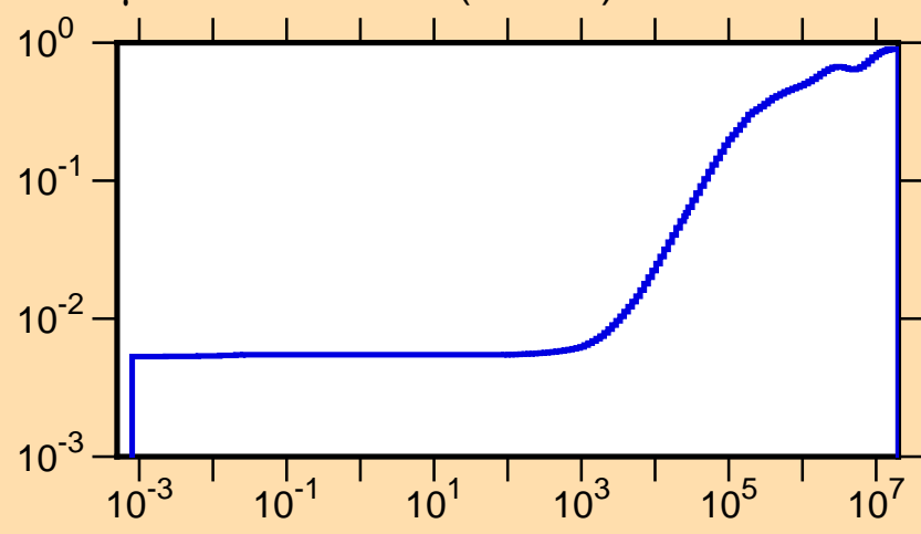
\mu vs. E for ^{127}\text{Te}(\text{mt251})
