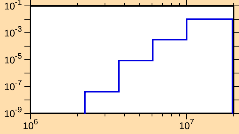
\sigma vs. E for ^{127}\text{Te}(n,p)
