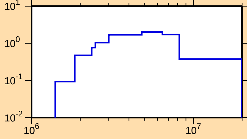
\sigma vs. E for ^{127}\text{Te}(n,n\text{cont.})
