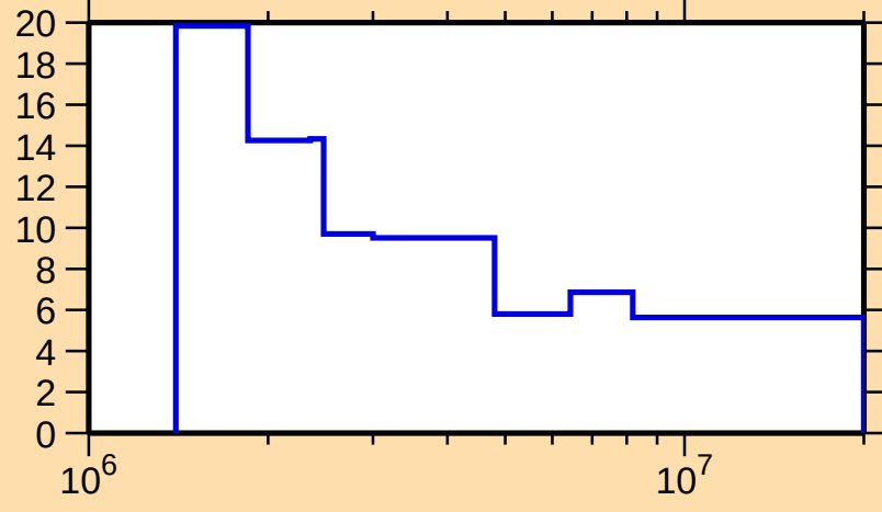
\Delta\sigma/\sigma vs. E for ^{127}\text{Te}(n,n\text{onel.})
