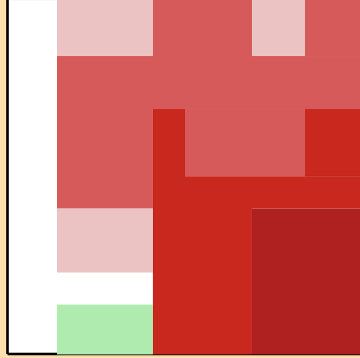
\Delta\sigma/\sigma vs. E for ^{127}\text{Te}(n,2n)
